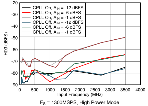
5-74. HD3 vs Input Frequency, CPLL and Input Amplitude
