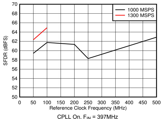
5-61. SFDR vs Reference Clock Frequency
