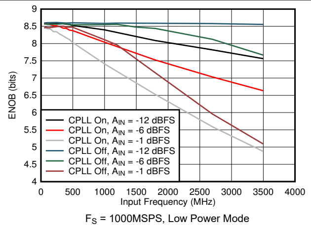
5-78. ENOB vs Input Frequency, CPLL and Input Amplitude
