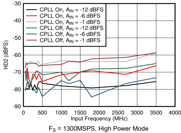
5-73. HD2 vs Input Frequency, CPLL and Input Amplitude
