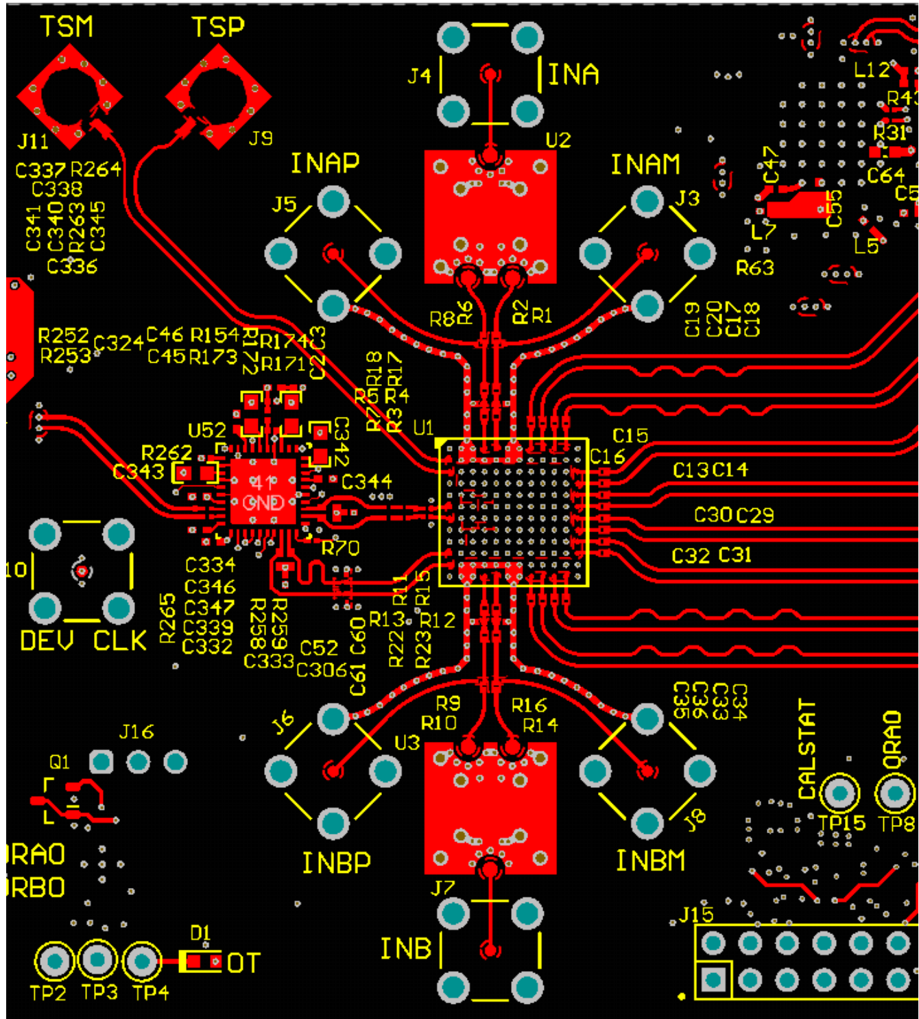
図 7-4. Top Layer Routing: Analog Inputs, CLK and SYSREF, DA0-3, DB0-3
