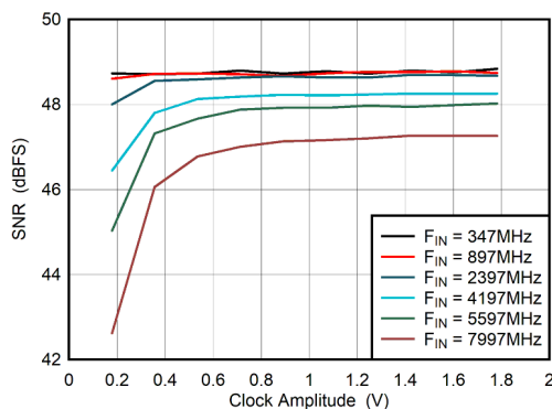
FIG 5-83. Dual Channel Mode: SNR vs Clock Amplitude
