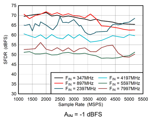
5-47. Dual Channel Mode: SFDR vs Sample Rate
