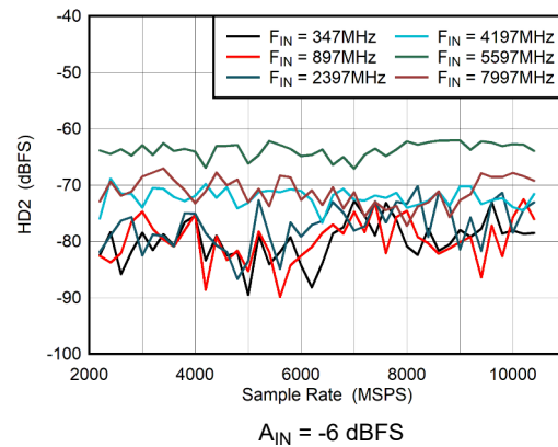
Figure 5-36. DES Mode: HD2 vs Sample Rate
