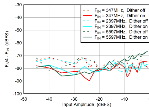
図 5-70. DES Mode: F_S/4 - F_{\text{IN}} vs Input Amplitude and Dither
