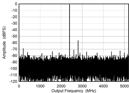
FIG 5-7. DES Mode: Single Tone FFT at 2397 MHz
