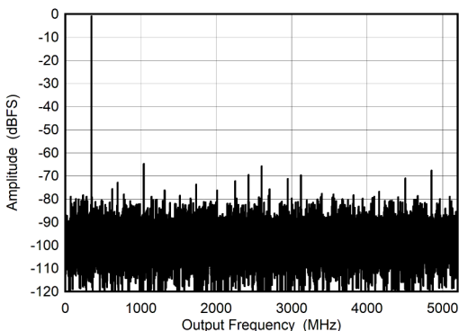
5-5. DES Mode: Single Tone FFT at 347 MHz
