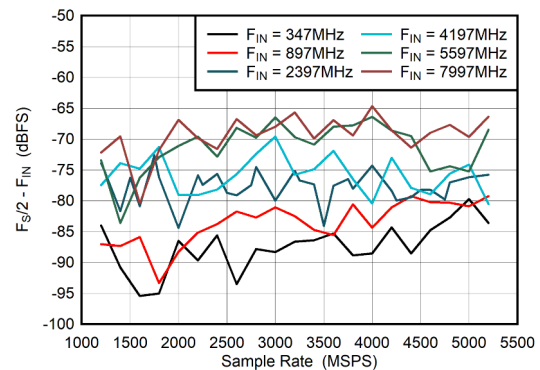
Figure 5-56. Dual Channel Mode: F_S/2 - F_{\text{IN}} vs Sample Rate
