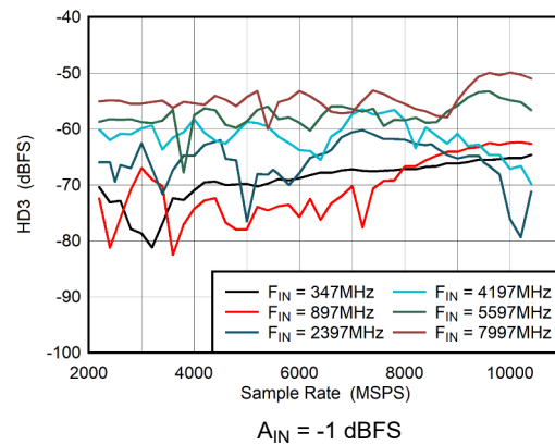
5-38. DES Mode: HD3 vs Sample Rate
