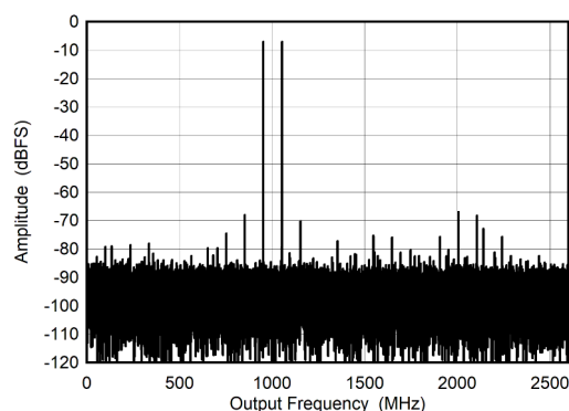
5-26. Dual Channel Mode: Two Tone FFT at 4197 MHz
