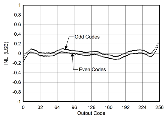
5-4. INL vs ADC Code
