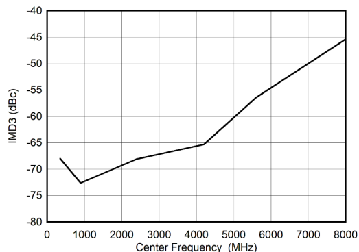
5-105. Dual Channel Mode: IMD3 vs Input Frequency
