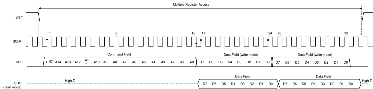
図 6-16. Serial Interface Protocol: Streaming Read/Write
