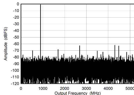
5-6. DES Mode: Single Tone FFT at 897 MHz
