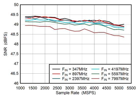
Figure 5-45. Dual Channel Mode: SNR vs Sample Rate
