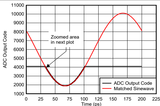
FIG 5-125. Sinewave Overdrive Recovery
