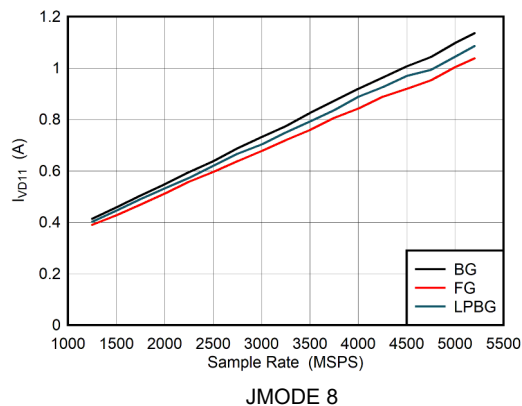
5-116. Dual Channel Mode: I_{VD11} vs Sample Rate
