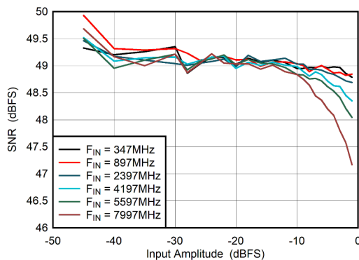
Figure 5-57. DES Mode: SNR vs Input Amplitude
