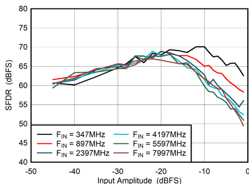
Figure 5-59. DES Mode: SFDR vs Input Amplitude
