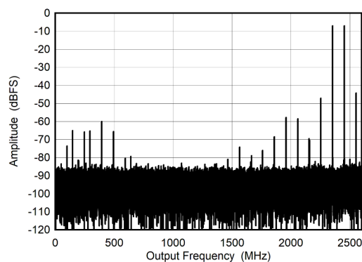
5-26. Dual Channel Mode: Two Tone FFT at 4197 MHz
