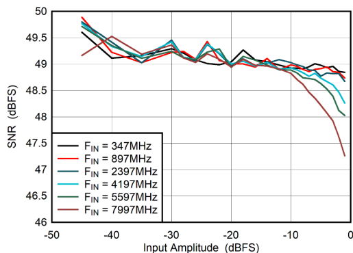
図 5-71. Dual Channel Mode: SNR vs Input Amplitude
