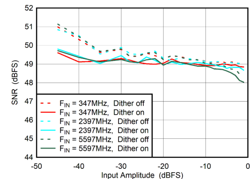
図 5-72. Dual Channel Mode: SNR vs Input Amplitude and Dither
