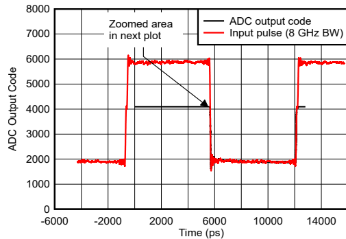
FIG 5-123. Pulse Overdrive Recovery
