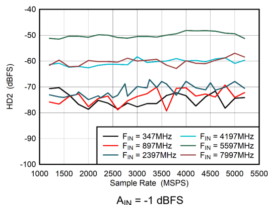
5-50. Dual Channel Mode: HD2 vs Sample Rate
