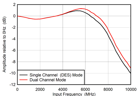
5-1. Input Amplitude vs Input Frequency
