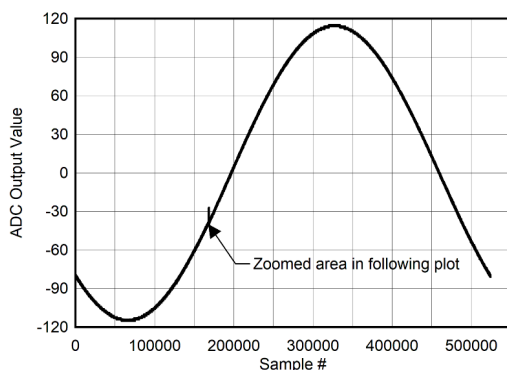
5-119. Background Calibration Core Transition (AC Signal)
