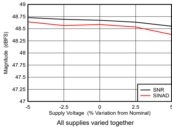
FIG 5-95. Dual Channel Mode: SNR and SINAD vs Supply Voltage
