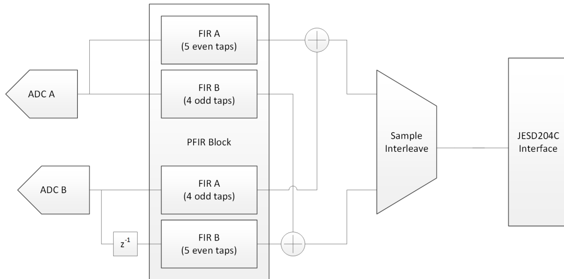
図 6-7. Alternate I/Q Correction-Type Filter Block Diagram
