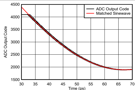
FIG 5-126. Sinewave Overdrive Recovery
