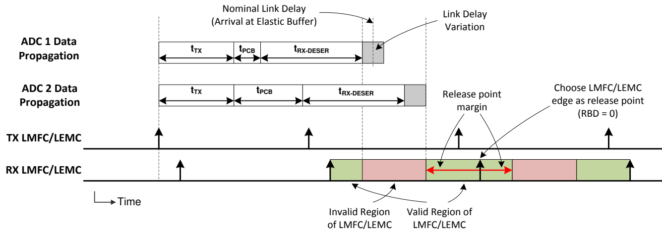
Figure 6-12. LMFC/LEMC Valid Region Definition for Elastic Buffer Release Point Selection
