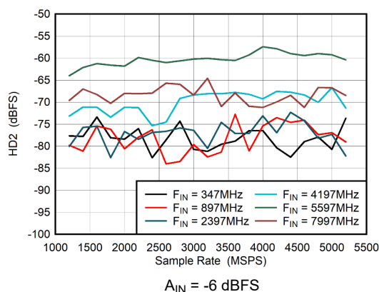
5-51. Dual Channel Mode: HD2 vs Sample Rate
