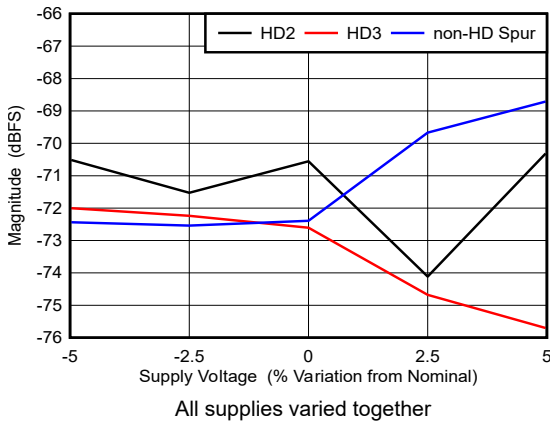
Figure 5-97. Dual Channel Mode: HD2, HD3 and Worst Spur vs Supply Voltage
