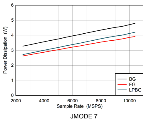
5-113. DES Mode: Power Dissipation vs Sample Rate
