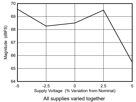
FIG 5-96. Dual Channel Mode: SFDR vs Supply Voltage
