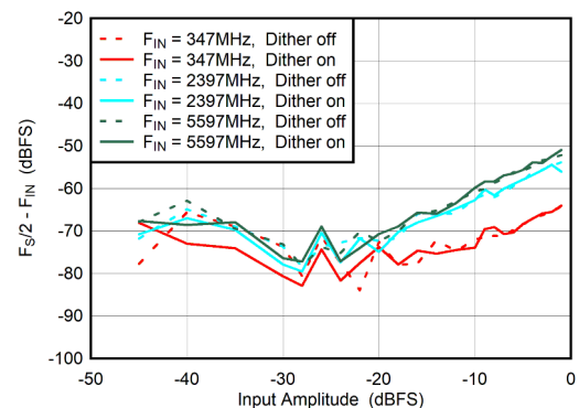
図 5-66. DES Mode: F_{\text{S}}/2 - F_{\text{IN}} vs Input Amplitude and Dither
