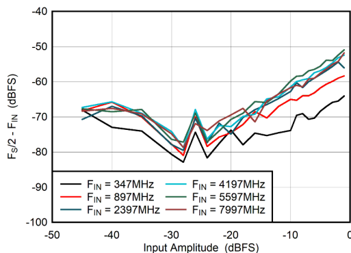
図 5-65. DES Mode: F_{\text{S}}/2 - F_{\text{IN}} vs Input Amplitude
