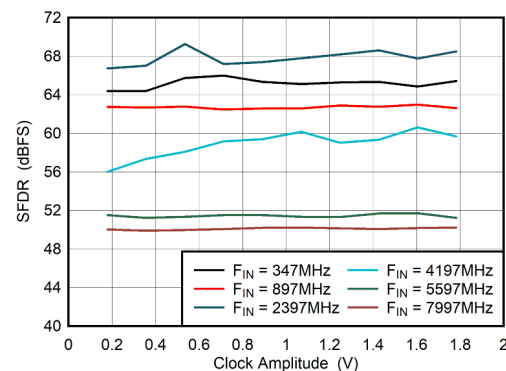
FIG 5-84. Dual Channel Mode: SFDR vs Clock Amplitude
