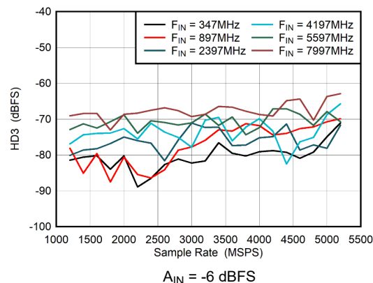
5-54. Dual Channel Mode: HD3 vs Sample Rate
