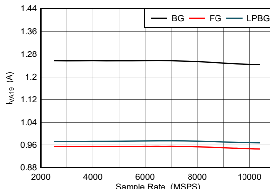
FIG 5-110. DES Mode: I_{VA19} vs Sample Rate
