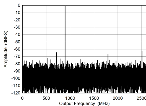
FIG 5-18. Dual Channel Mode: Single Tone FFT at 897 MHz
