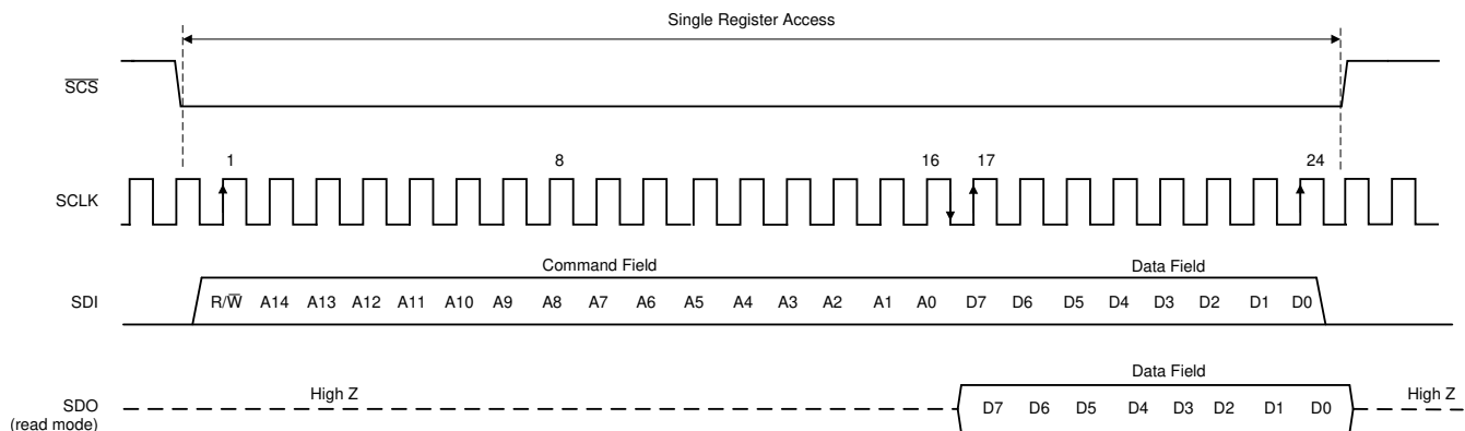
Figure 6-15. Serial Interface Protocol: Single Read/Write
