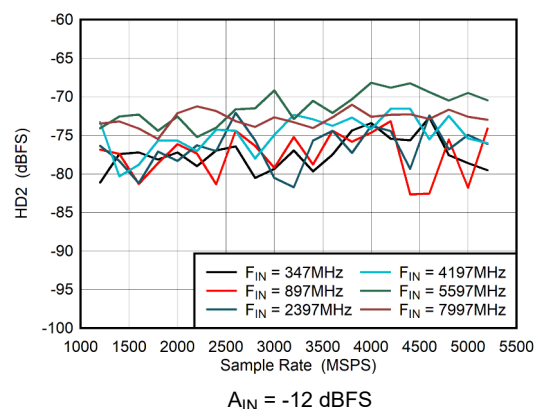
5-52. Dual Channel Mode: HD2 vs Sample Rate
