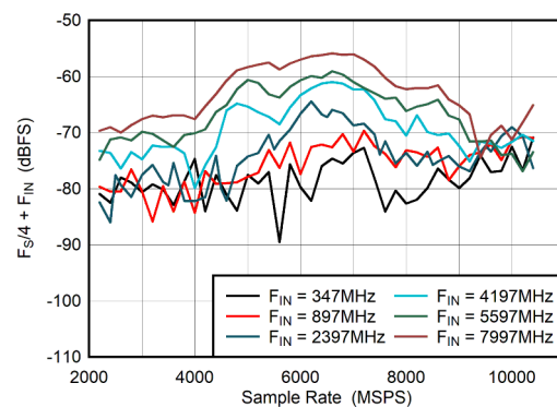
5-42. DES Mode: F_S/4 + F_{\text{IN}} vs Sample Rate
