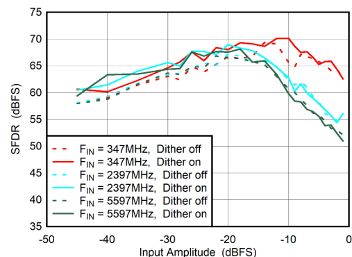
Figure 5-60. DES Mode: SFDR vs Input Amplitude and Dither
