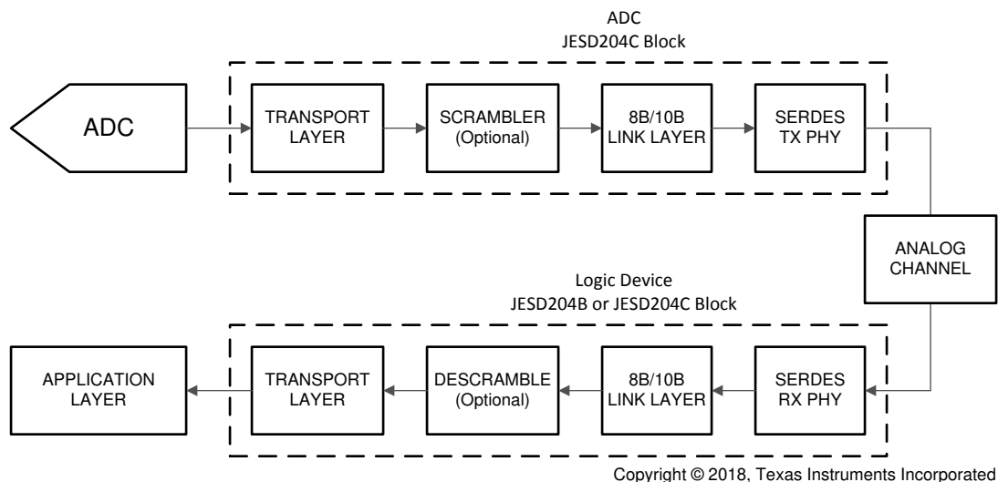
図 6-8. Simplified 8B/10B Encoded JESD204C Interface Diagram
