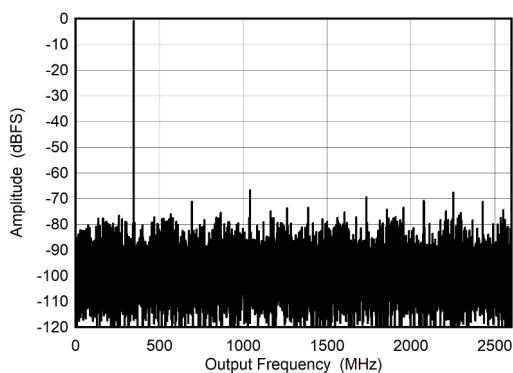
FIG 5-17. Dual Channel Mode: Single Tone FFT at 347 MHz
