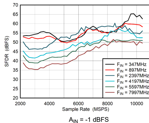
5-32. DES Mode: SFDR vs Sample Rate
