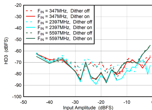
Figure 5-78. Dual Channel Mode: HD3 vs Input Amplitude and Dither
