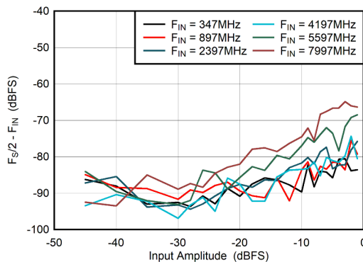
FIG 5-79. Dual Channel Mode: F_{\text{S}}/2 - F_{\text{IN}} vs Input Amplitude
