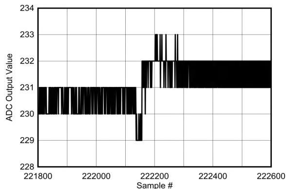
5-122. Background Calibration Core Transition (DC Signal Zoomed)
