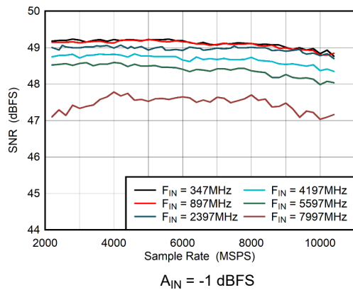
5-29. DES Mode: SNR vs Sample Rate
