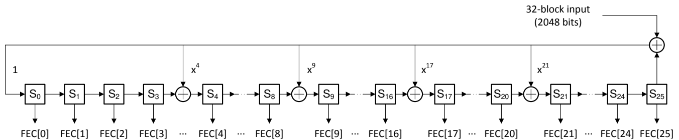
❏ 6-11. FEC Parity Bit Generator
