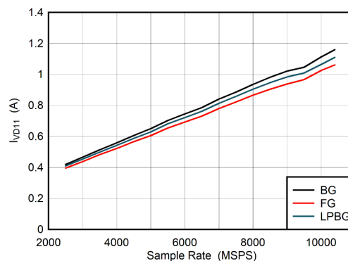
FIG 5-112. DES Mode: I_{VD11} vs Sample Rate
