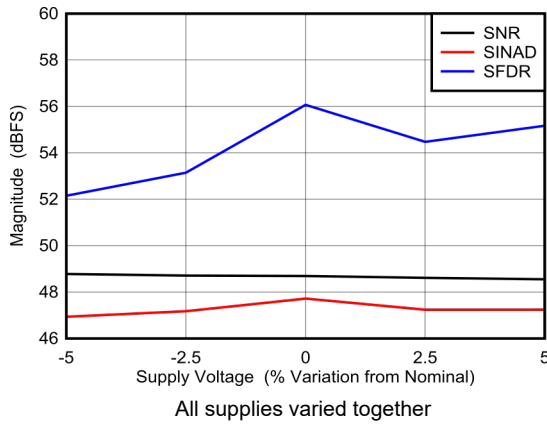
FIG 5-93. DES Mode: SNR, SINAD and SFDR vs Supply Voltage
