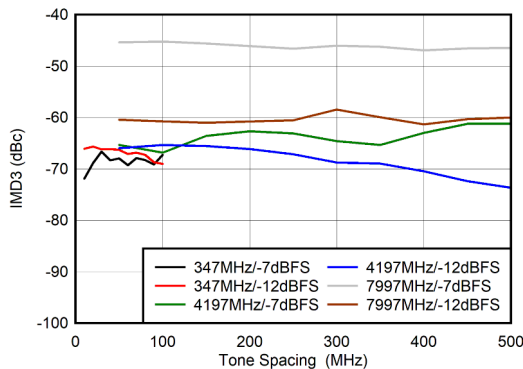
5-107. Dual Channel Mode: IMD3 vs Tone Spacing
