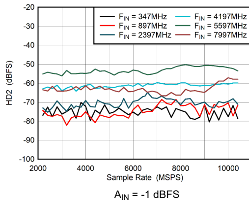
Figure 5-35. DES Mode: HD2 vs Sample Rate
