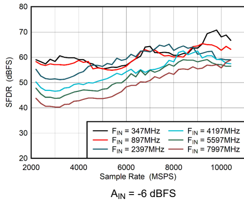
Figure 5-33. DES Mode: SFDR vs Sample Rate
