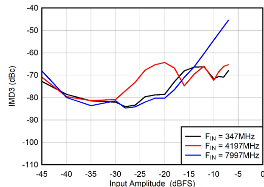
5-106. Dual Channel Mode: IMD3 vs Input Amplitude
