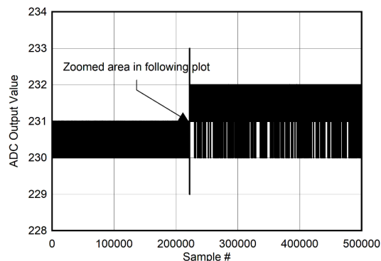
5-121. Background Calibration Core Transition (DC Signal)
