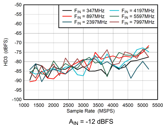
Figure 5-55. Dual Channel Mode: HD3 vs Sample Rate
