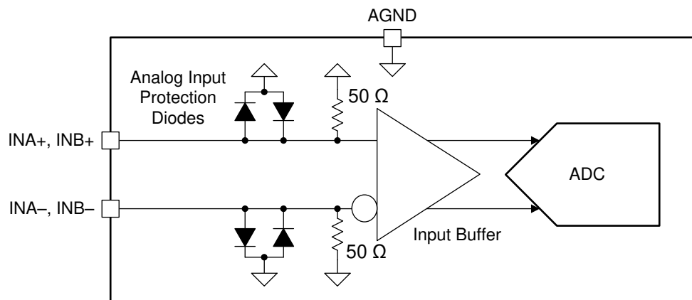
図 6-1. ADC08DJ5200RF Analog Input Internal Termination and Protection Diagram
