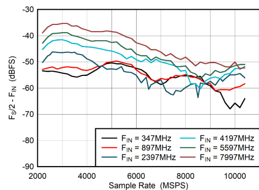
5-41. DES Mode: F_S/2 - F_{\text{IN}} vs Sample Rate
