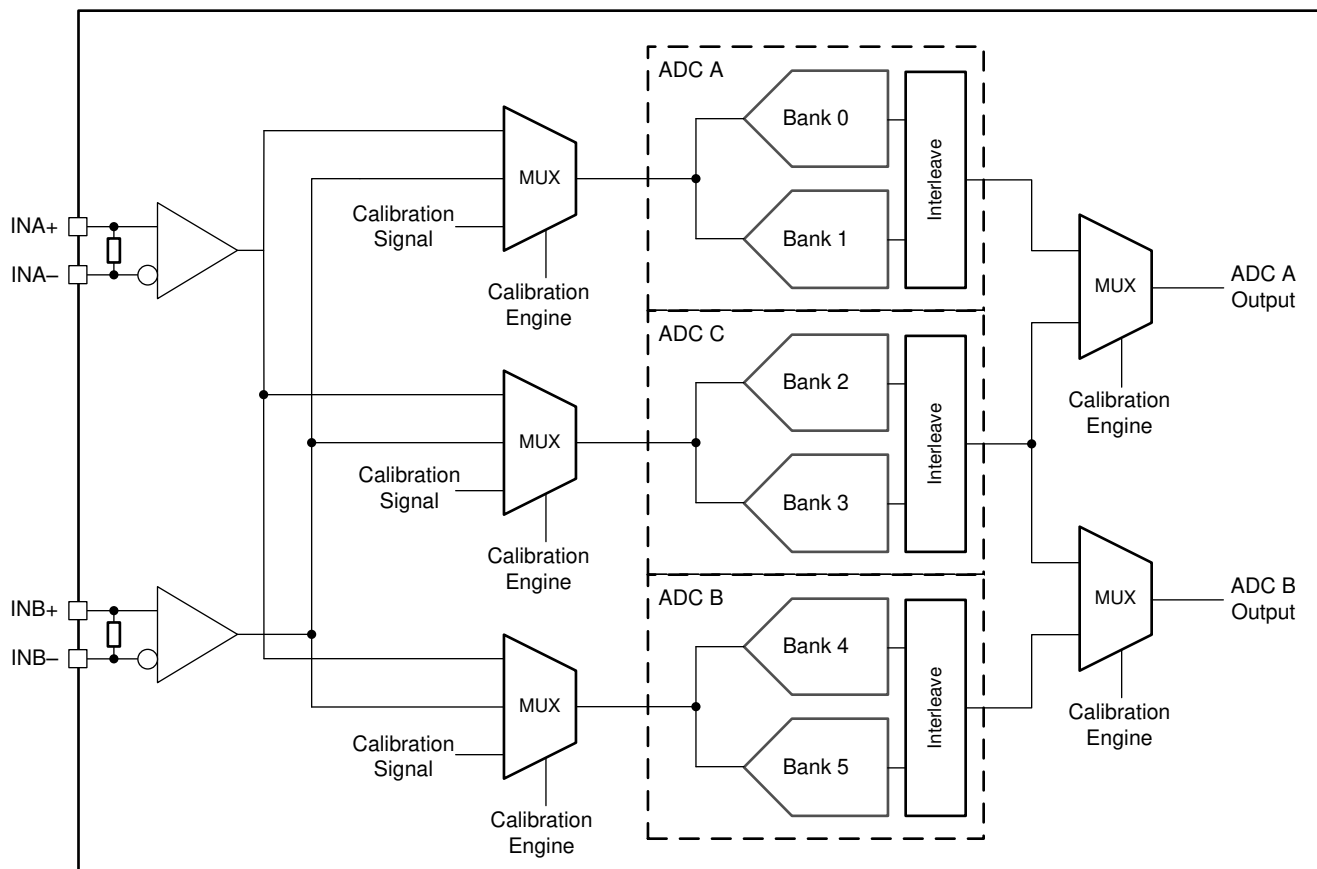
図 6-14. ADC08DJ5200RF Calibration System Block Diagram
