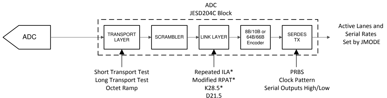
Figure 6-13. Test Mode Insertion Points
