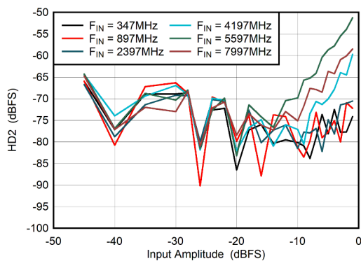
Figure 5-75. Dual Channel Mode: HD2 vs Input Amplitude
