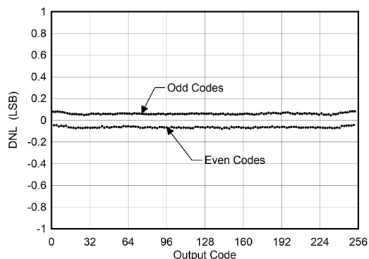
5-3. DNL vs ADC Code
