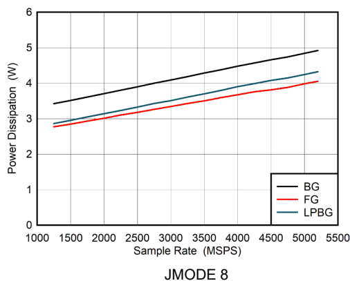
5-117. Dual Channel Mode: Power Dissipation vs Sample Rate
