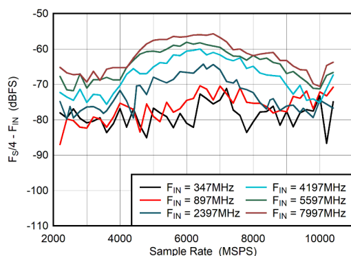
Figure 5-43. DES Mode: F_S/4 - F_{\text{IN}} vs Sample Rate
