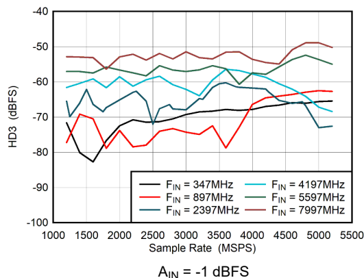
5-53. Dual Channel Mode: HD3 vs Sample Rate
