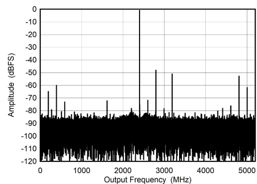
FIG 5-10. DES Mode: Single Tone FFT at 7997 MHz
