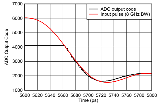
FIG 5-124. Pulse Overdrive Recovery Zoomed
