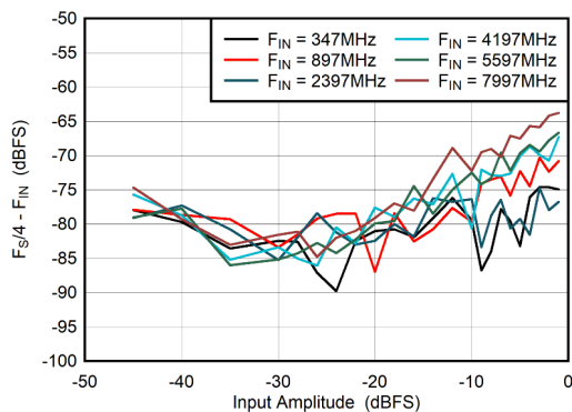
図 5-69. DES Mode: F_S/4 - F_{\text{IN}} vs Input Amplitude
