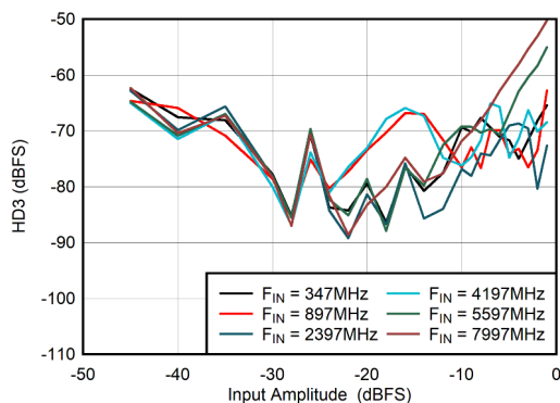
Figure 5-77. Dual Channel Mode: HD3 vs Input Amplitude
