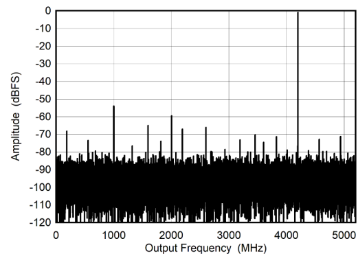
FIG 5-8. DES Mode: Single Tone FFT at 4197 MHz
