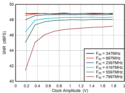
FIG 5-81. DES Mode: SNR vs Clock Amplitude
