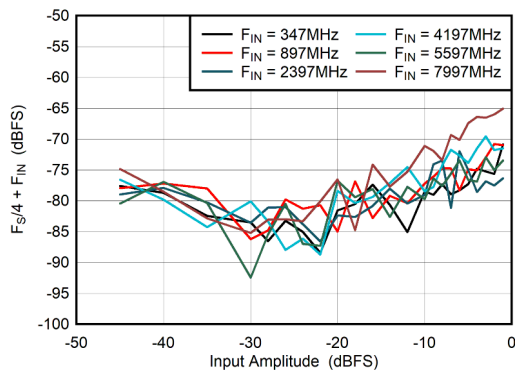
図 5-67. DES Mode: F_S/4 + F_{\text{IN}} vs Input Amplitude
