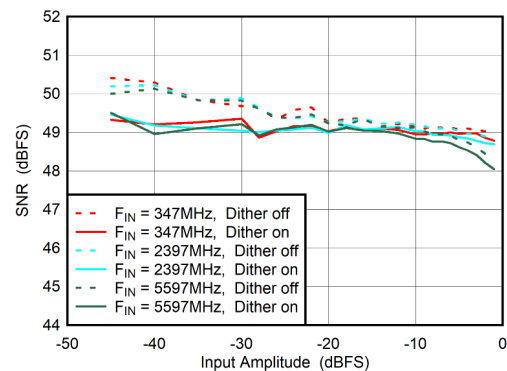
Figure 5-58. DES Mode: SNR vs Input Amplitude and Dither
