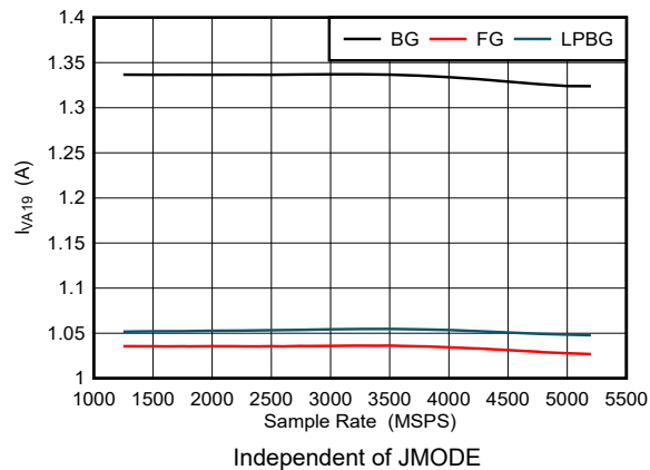
5-114. Dual Channel Mode: I_{VA19} vs Sample Rate
