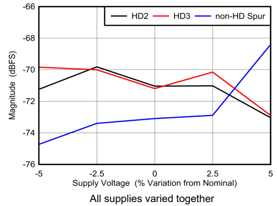
FIG 5-94. DES Mode: HD2, HD3 and Worst Spur vs Supply Voltage
