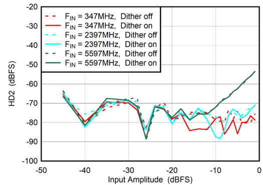
図 5-62. DES Mode: HD2 vs Input Amplitude and Dither
