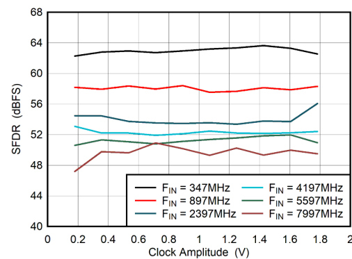
FIG 5-82. DES Mode: SFDR vs Clock Amplitude
