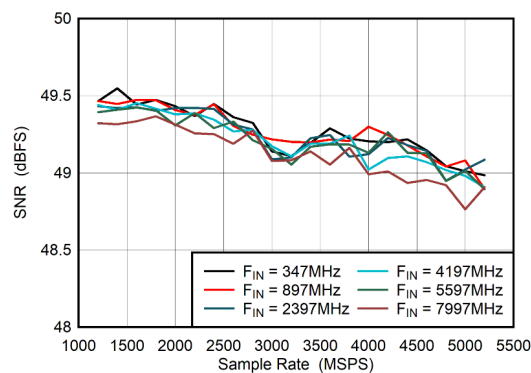
Figure 5-44. Dual Channel Mode: SNR vs Sample Rate
