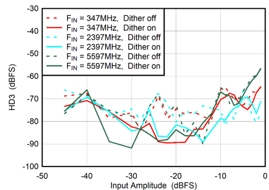
図 5-64. DES Mode: HD3 vs Input Amplitude and Dither
