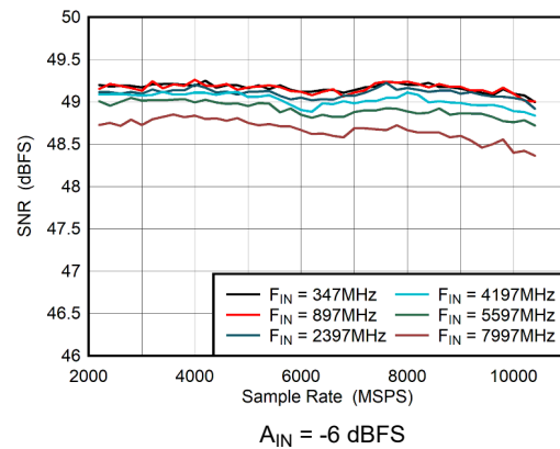
5-30. DES Mode: SNR vs Sample Rate
