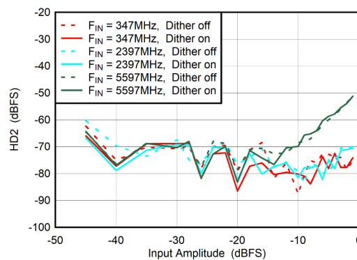
Figure 5-76. Dual Channel Mode: HD2 vs Input Amplitude and Dither
