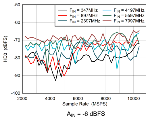
5-39. DES Mode: HD3 vs Sample Rate
