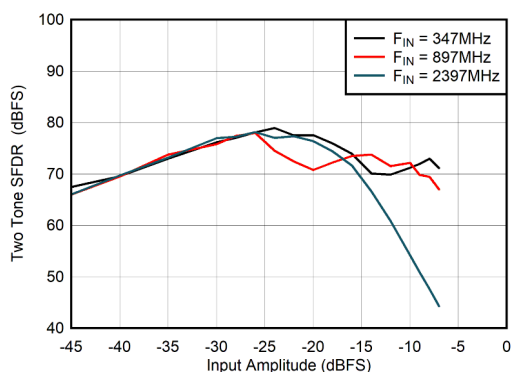
FIG 5-109. Dual Channel Mode: Two Tone SFDR vs Input Amplitude
