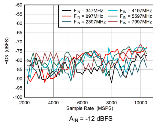
5-40. DES Mode: HD3 vs Sample Rate
