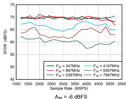
5-48. Dual Channel Mode: SFDR vs Sample Rate
