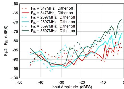
FIG 5-80. Dual Channel Mode: F_{\text{S}}/2 - F_{\text{IN}} vs Input Amplitude and Dither
