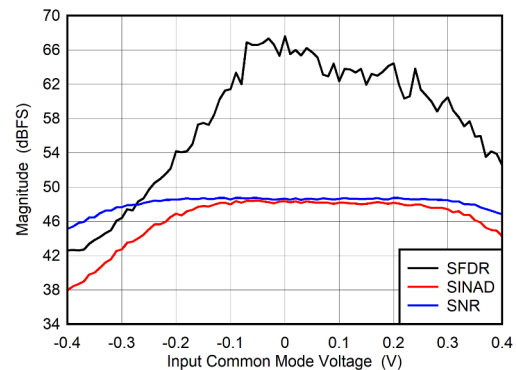
Figure 5-98. DES Mode: SNR, SFDR and SINAD vs Input Common Mode Voltage
