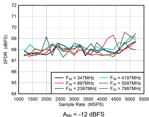
5-49. Dual Channel Mode: SFDR vs Sample Rate
