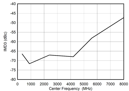
Figure 5-100. DES Mode: IMD3 vs Input Frequency
