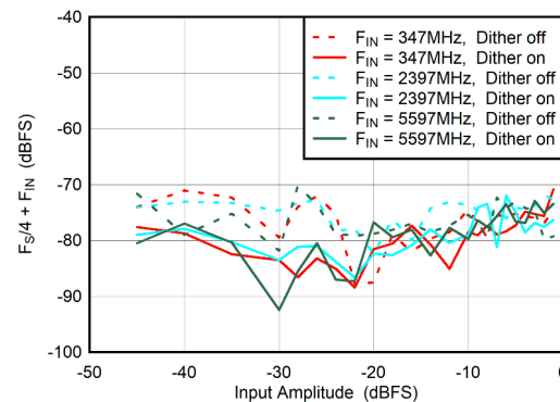
図 5-68. DES Mode: F_S/4 + F_{\text{IN}} vs Input Amplitude and Dither
