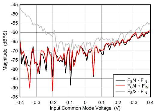
Figure 5-99. DES Mode: F_S/2 - F_{\text{IN}} , F_S/4 \pm F_{\text{IN}} vs Input Common Mode Voltage
