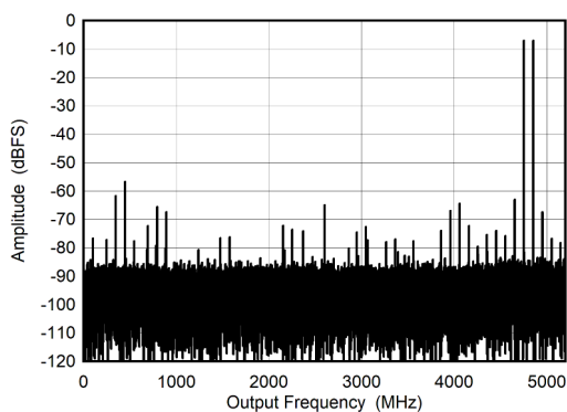
FIG 5-13. DES Mode: Two Tone FFT at 2397 MHz
