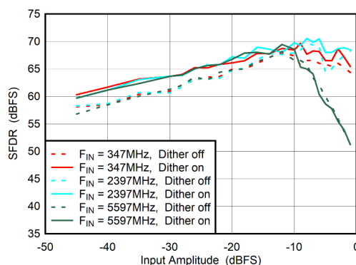
Figure 5-74. Dual Channel Mode: SFDR vs Input Amplitude and Dither
