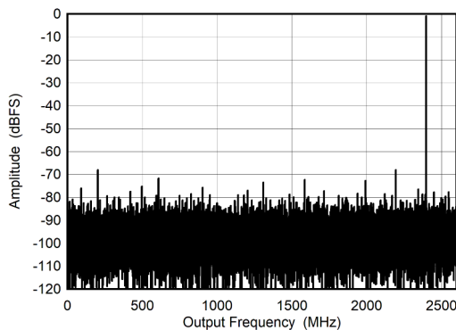
Figure 5-19. Dual Channel Mode: Single Tone FFT at 2397 MHz
