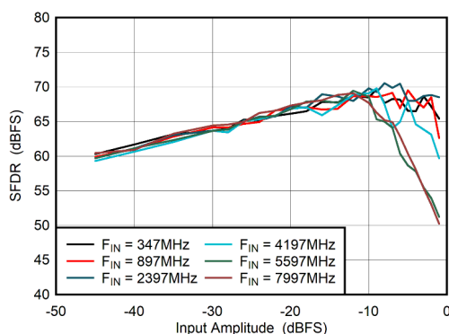
Figure 5-73. Dual Channel Mode: SFDR vs Input Amplitude
