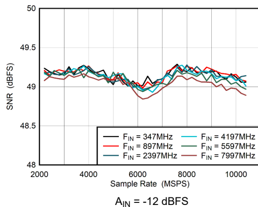
5-31. DES Mode: SNR vs Sample Rate
