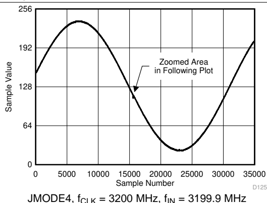
Figure 58. Background Calibration Core Transition (AC Signal)
