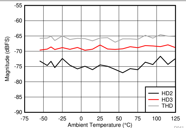
JMODE5, f_S = 6400\text{ MSPS} , f_{IN} = 2400\text{ MHz} , BG calibration
