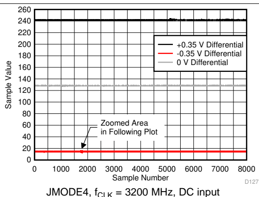
Figure 60. Background Calibration Core Transition (DC Signal)
