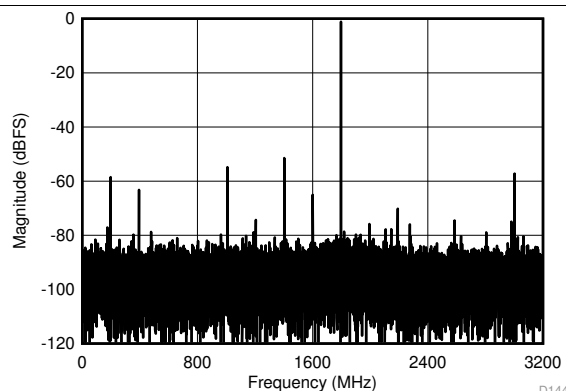
JMODE5, f_{\text{IN}} = 8200\text{ MHz} , FG calibration, SNR = 47.4 dBFS, SFDR = 51.4 dBFS, ENOB = 7.10 bits
