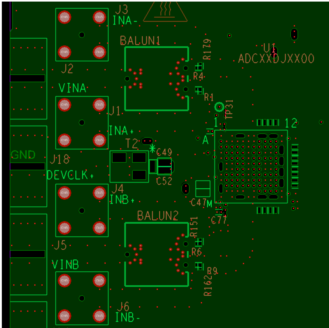
✎ 169. GND1 Cutouts to Optimize Impedance of Component Pads
