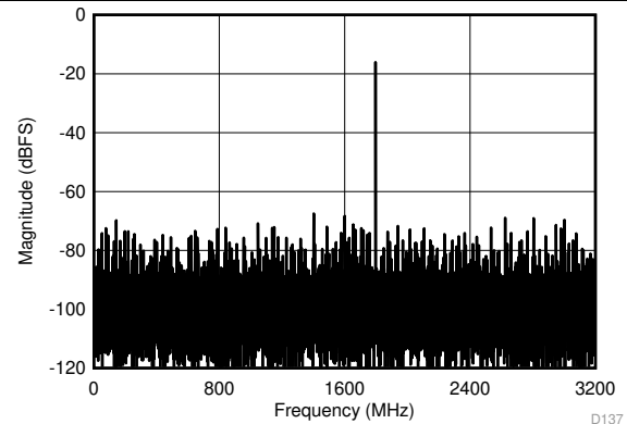
JMODE5, f_{IN} = 8200\text{ MHz} , FG calibration, SNR = 49.0 dBFS, SFDR = 67.5 dBFS, ENOB = 7.79 bits
