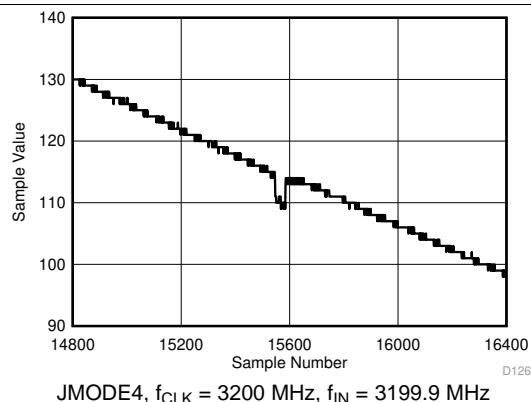
Figure 59. Background Calibration Core Transition (AC Signal Zoomed)
