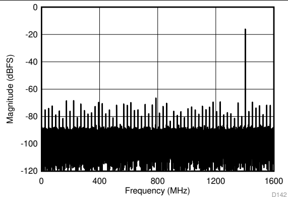
JMODE7, f_{IN} = 8200\text{ MHz} , FG calibration, SNR = 49.2 dBFS, SFDR = 65.9 dBFS, ENOB = 7.80 bits
