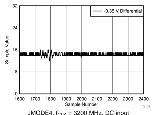
Figure 61. Background Calibration Core Transition (DC Signal Zoomed)
