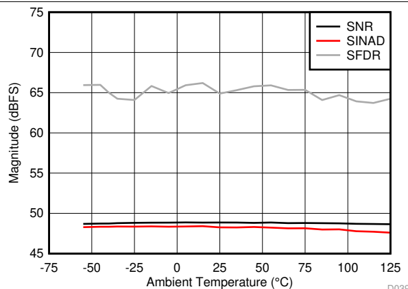
JMODE5, f_S = 6400\text{ MSPS} , f_{IN} = 2400\text{ MHz} , BG calibration
