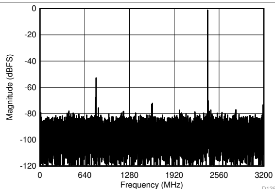
JMODE5, f_{\text{IN}} = 2400\text{ MHz} , FG calibration, SNR = 48.8 dBFS, SFDR = 52.4 dBFS, ENOB = 7.53 bits
