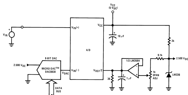
Figure 56. 1-mV Resolution With µP-Controlled Range
