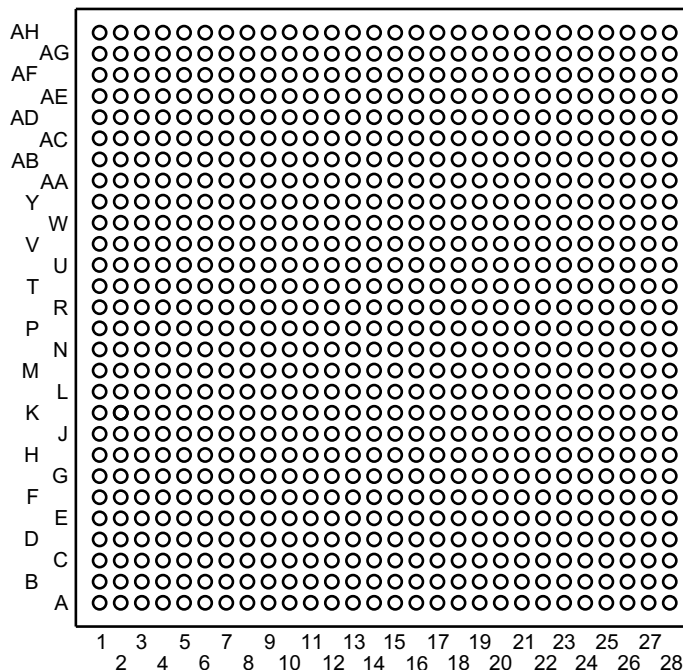
図 5-1. ACD FCBGA-N784 Package (Bottom View)
