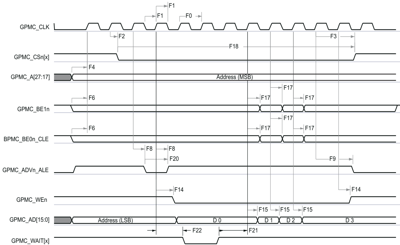
6-51. GPMC and Multiplexed NOR Flash—Synchronous Burst Read
