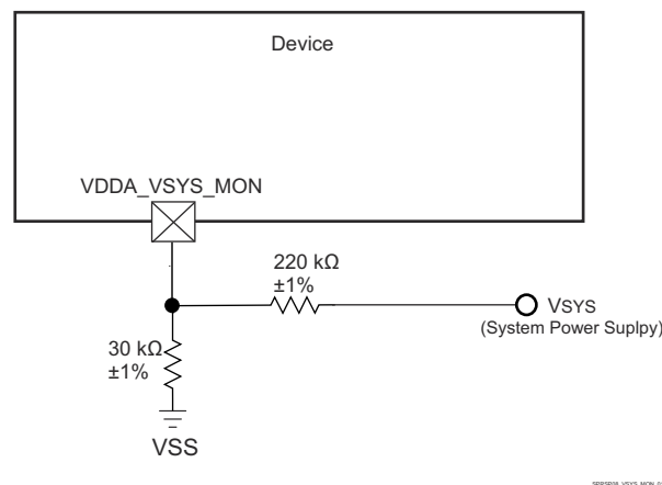
図 8-5. System Supply Monitor Voltage Divider Circuit
