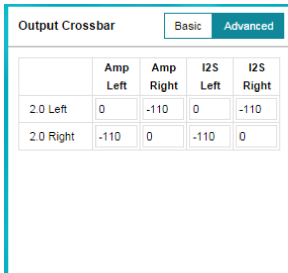
图 3-20. 输出交叉开关 (“Advanced (高级)”选项卡)
