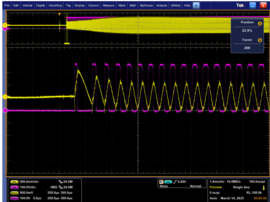
图 3-3. 满载 (15A) 启动 ( Ch1 = ISNS ; Ch3 = SW )
