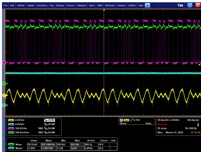
图 3-11. 3.5A 负载时的稳态波形 ( Ch1= ISNS ; Ch2 = Vout ; Ch3 = SW ; Ch4 = I_OPT )
