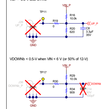
SEQUENCE UP/DOWN Inputs (0 - 7V)
