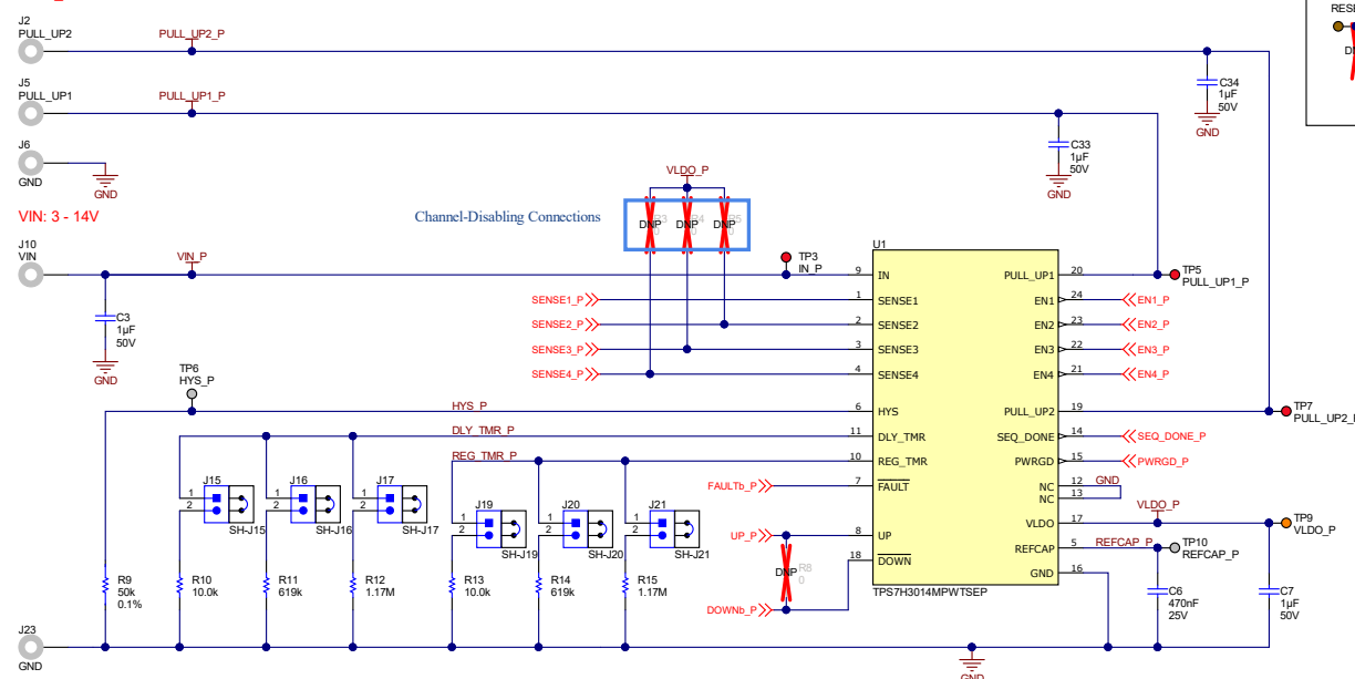
SENSE x Inputs of U1 (VSENSE x = 0 - 3.5V)
