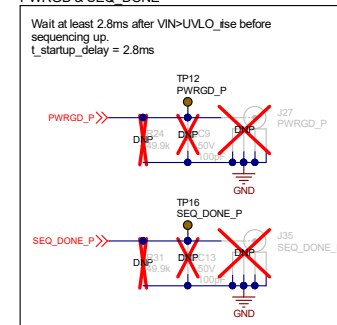
PWRGD &amp; SEQ_DONE
