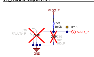
SR_FAULTb Output of U1
