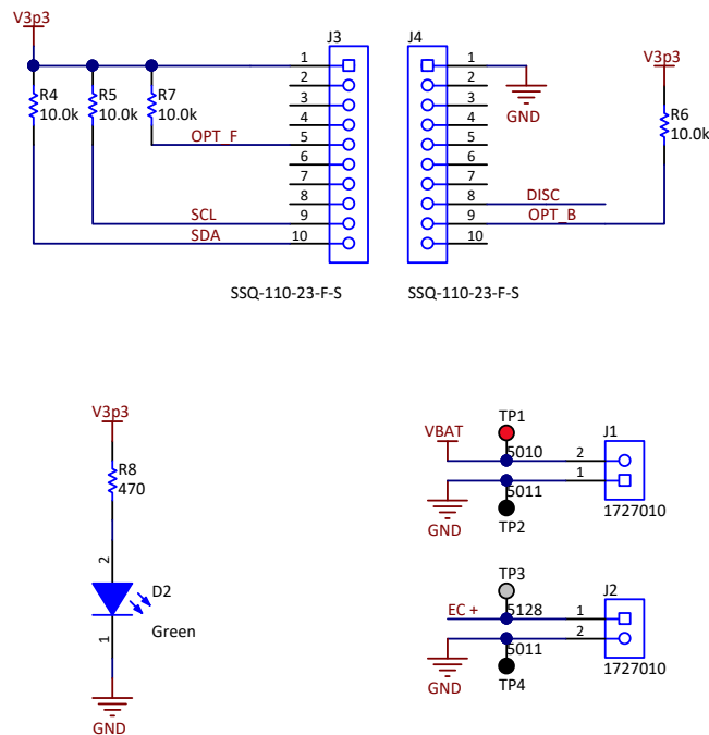
图 12. Schematic of Jumper Connections
