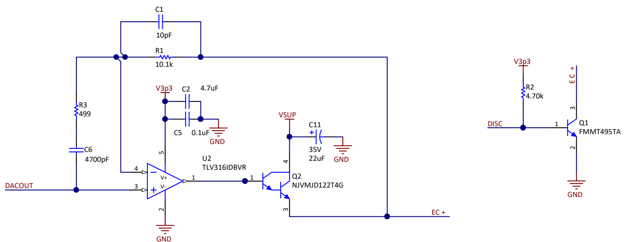
图 10. EC Mirror Driver Schematic
