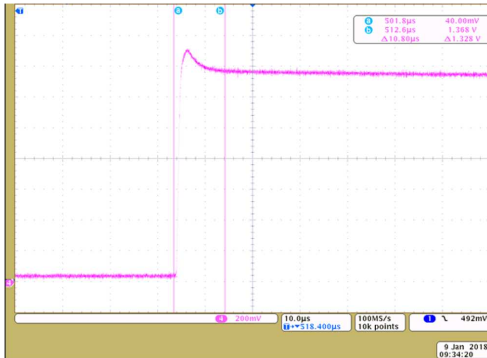
图 15. Impulse Response of EC Mirror Driver Stage With Typical Electrochromic Load
