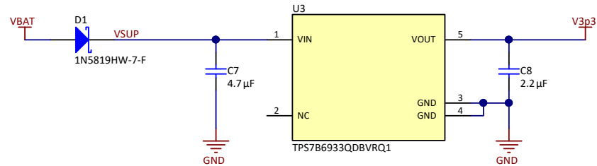
图 11. LDO Configuration Schematic
