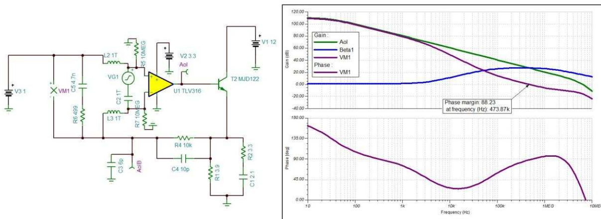
图 9. TINA-TI™ Stability Analysis of EC Mirror Driver With Compensation
