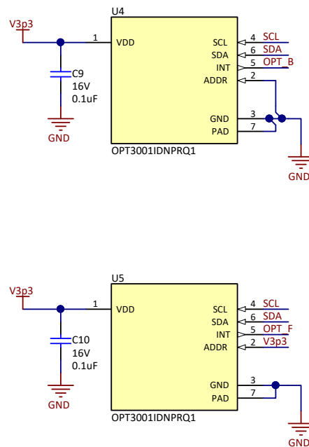
图 6. Ambient Light Sensors Schematic
