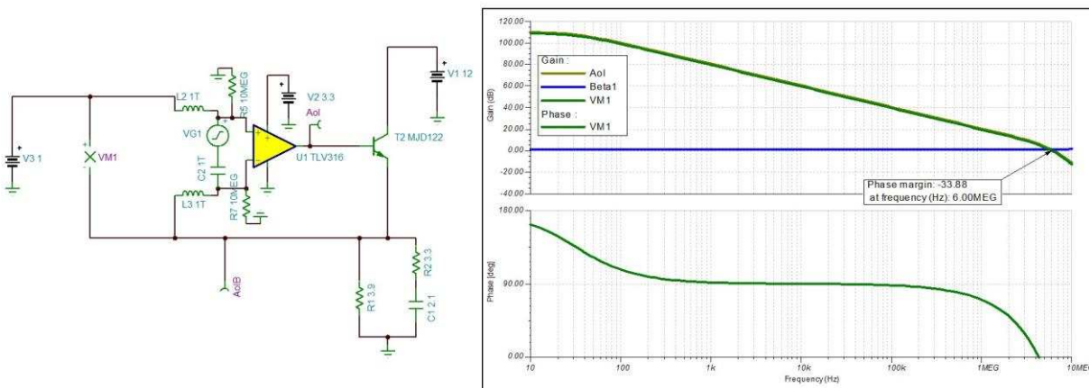
图 8. TINA-TI™ Stability Analysis of EC Mirror Driver Without Compensation
