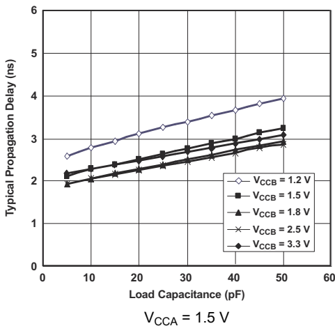
图 5-3. Typical Propagation Delay (A to B) vs Load Capacitance
