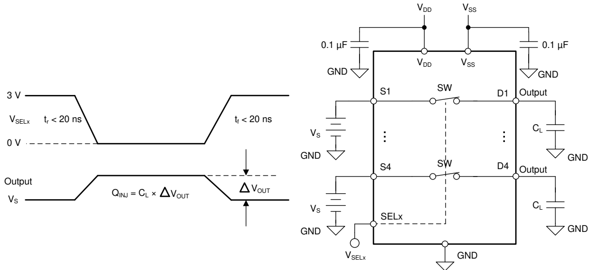
图 8-5. Charge-Injection Measurement Setup
