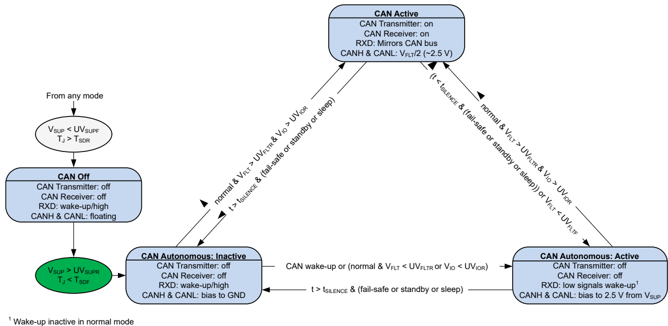
图 9-8. TCAN1162 CAN Transceiver State Machine
