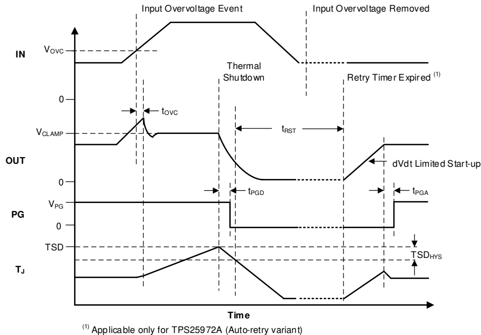
8-8. TPS25972x Overvoltage Response (Auto-Retry)
