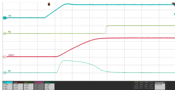
图 7-31. Power Up and Down With Input Supply
