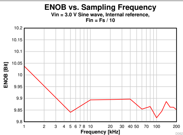
图 7-24. ENOB vs. Sampling Frequency
