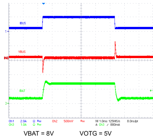
图 10-17. VOTG Load Transient Response
