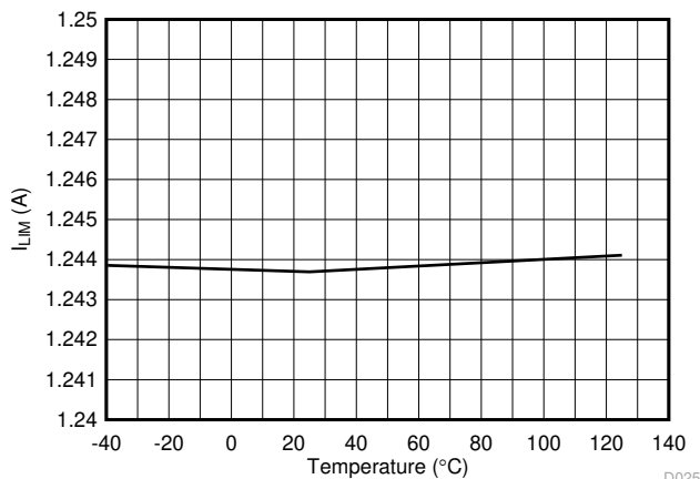
图 7-23. 2x Mode (2xFBn = 1) Current Limit vs Temperature
