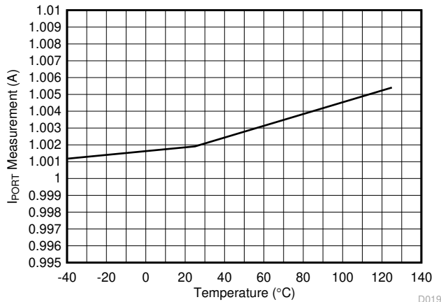
图 7-19. Port Current ADC Measurement (1 A) vs Temperature
