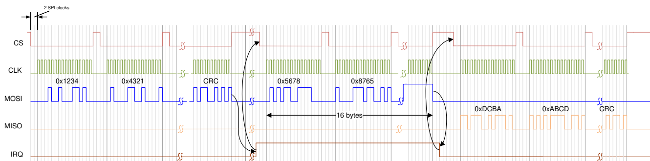
图 8-12. SPI Communication
