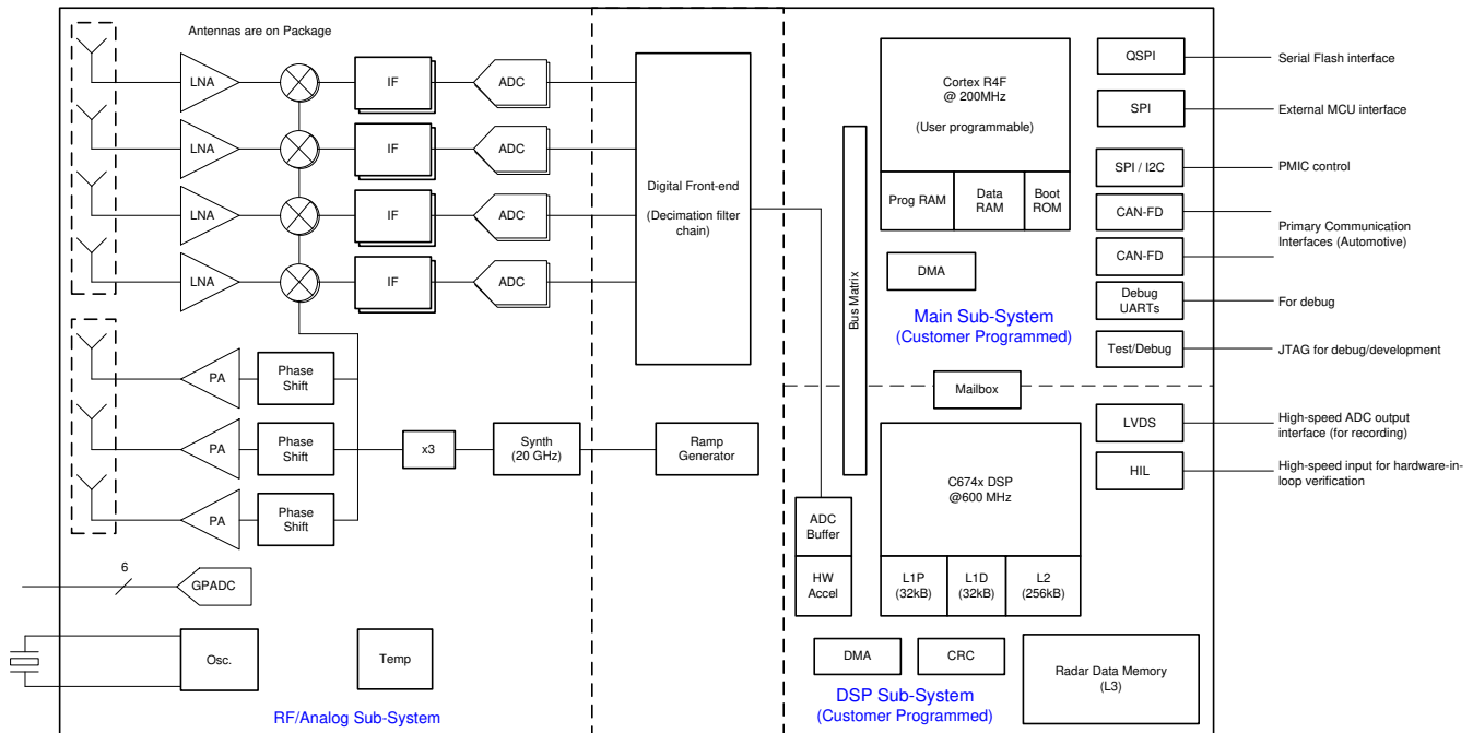
图 9-1. Functional Block Diagram
