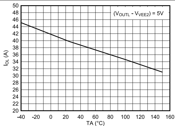
图 6-2. I_{O_{UL}} vs. Temperature
