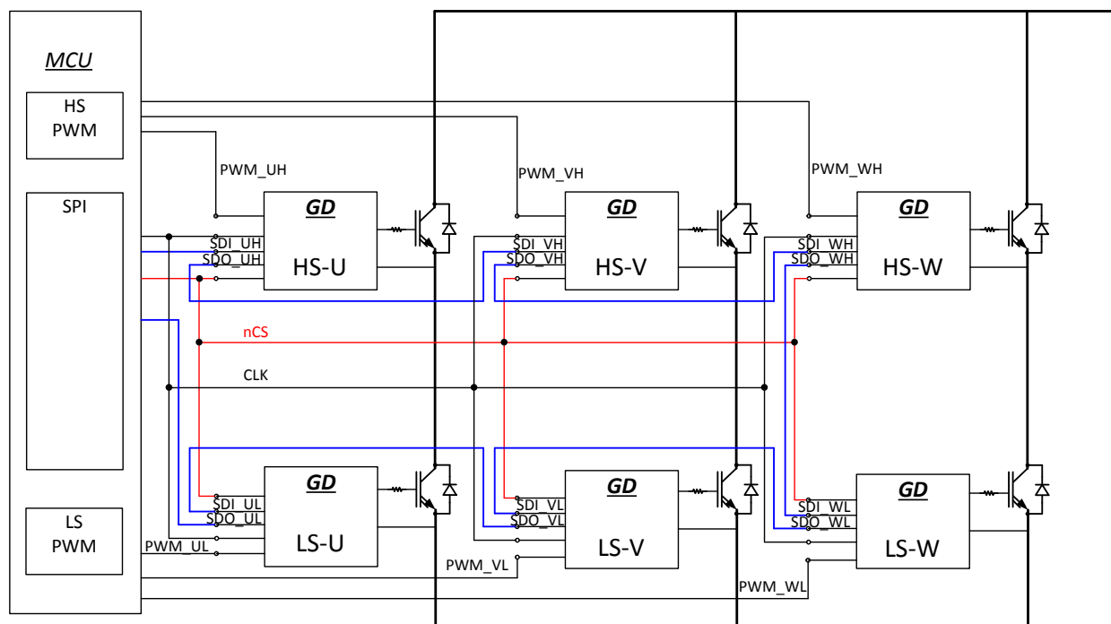
图 7-40. System configuration of daisy chain SPI configuration
