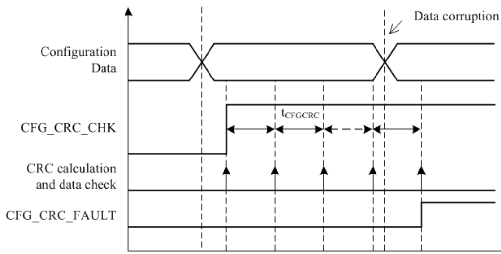
图 7-35. Configuration Data CRC Check Timing
