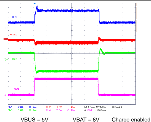
图 10-8. IINDPM Transient Response
