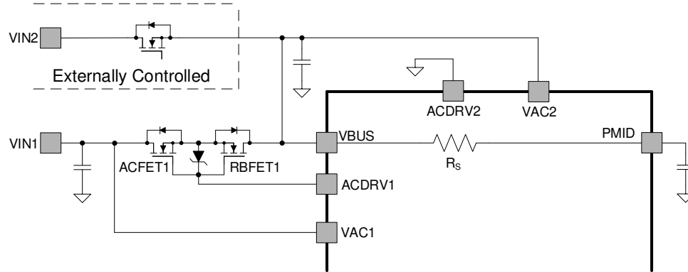
图 9-3. One ACFET-RBFET Structure Supporting One Input at VAC1 and/or One Input at VBUS
