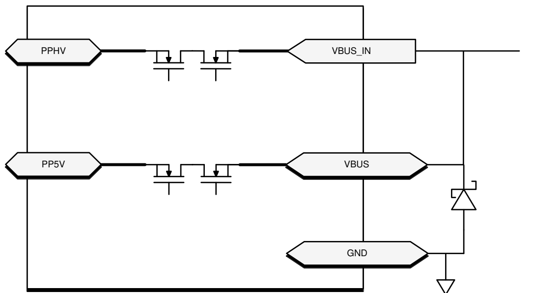
图 9-33. TPS25750D Schottky for Current Surge Protection
