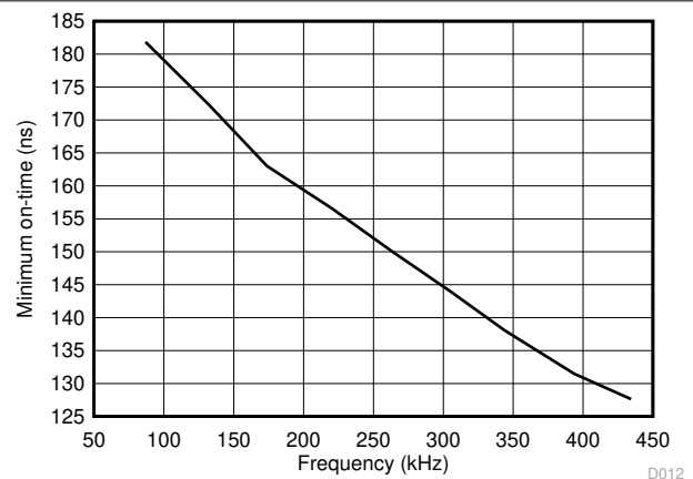
图 7-12. t_{\text{ON(MIN)}} vs Frequency
