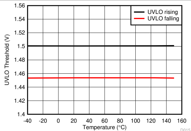
图 7-14. UVLO Threshold vs Temperature
