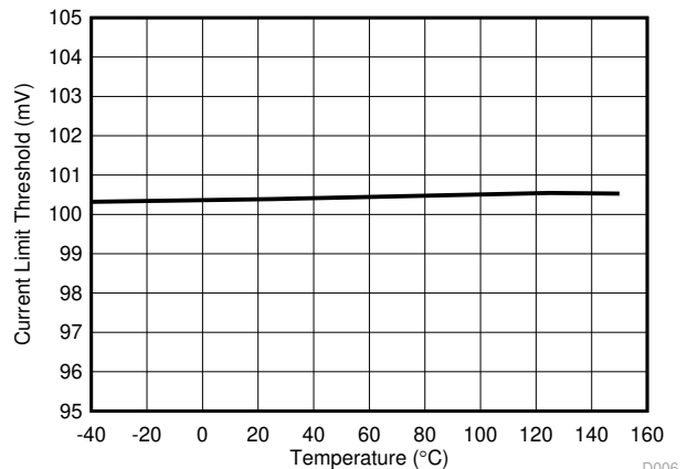
图 7-6. Current Limit Threshold vs Temperature
