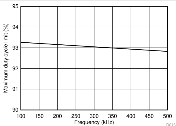
图 7-15. Maximum Duty Cycle vs Frequency
