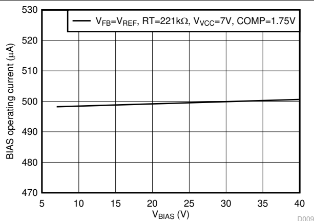
图 7-9. I_{\text{OPERATING(BIAS)}} Including RT Current vs V_{\text{BIAS}}
