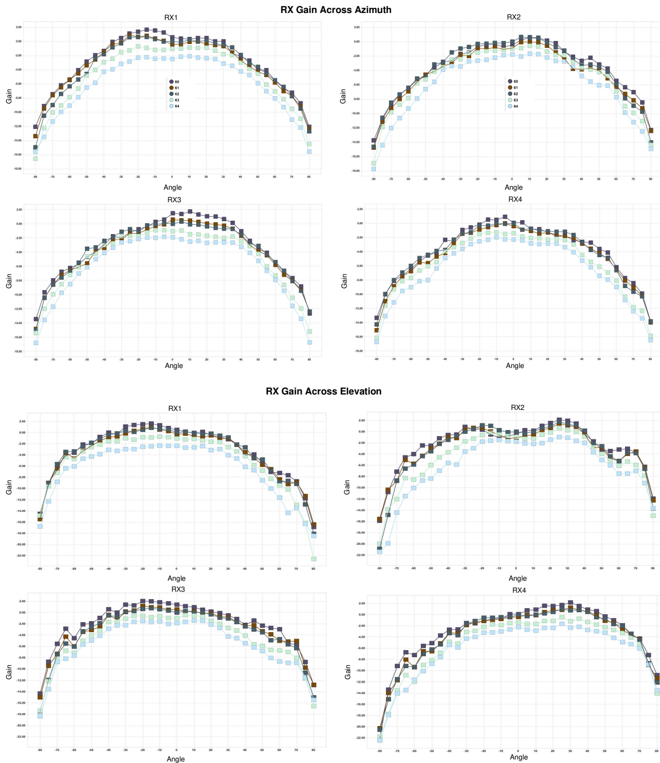
图 8-1. Receiver Antenna Radiation Pattern
