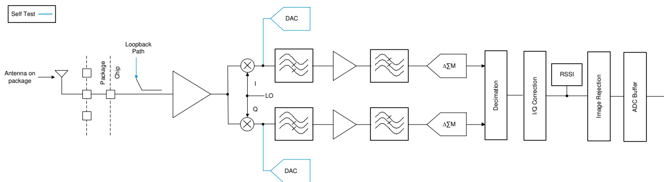
图 9-4. Receive Subsystem (Per Channel)
