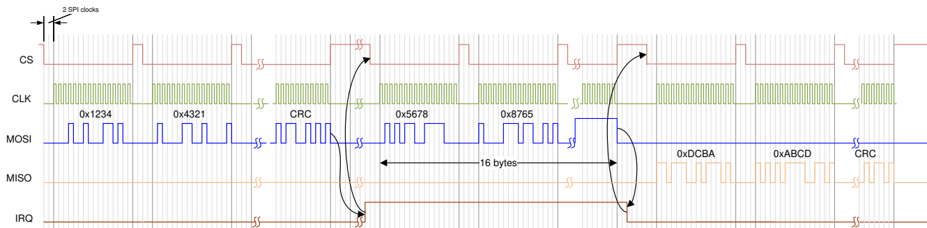
图 8-12. SPI Communication
