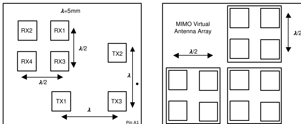
8-3. Antenna Positions (Placement and Relative Spacing)
