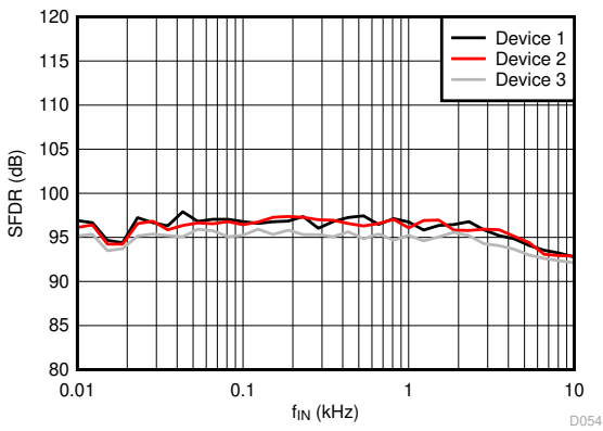
图 6-30. Spurious-Free Dynamic Range vs Input Signal Frequency
