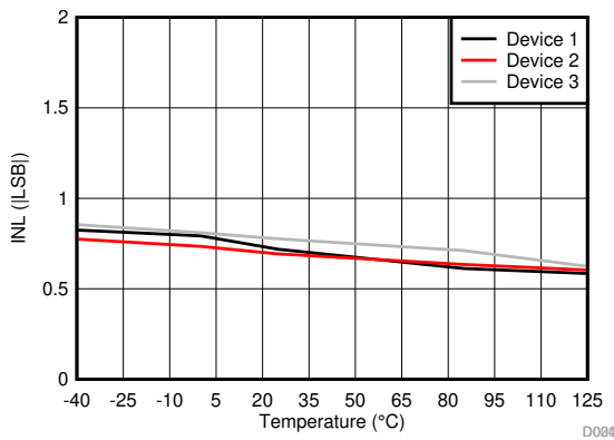
图 6-18. Integral Nonlinearity vs Temperature
