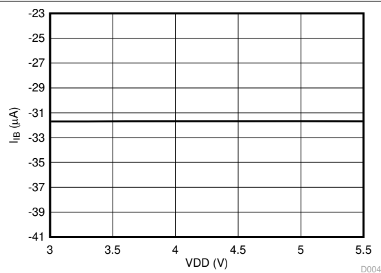
图 6-7. Input Bias Current vs Supply Voltage
