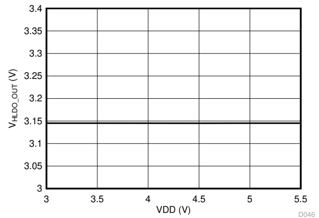
图 5-36. High-Side LDO Line Regulation
