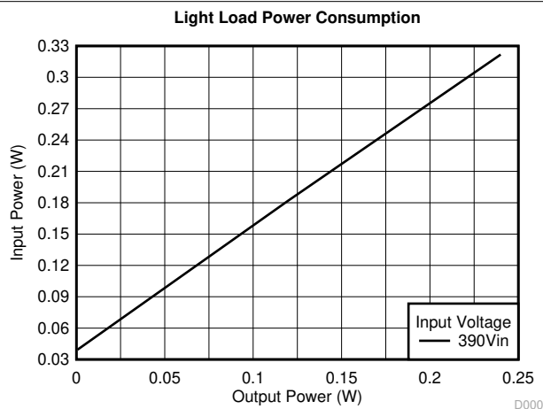
图 8-2. Light Load Power Consumption
