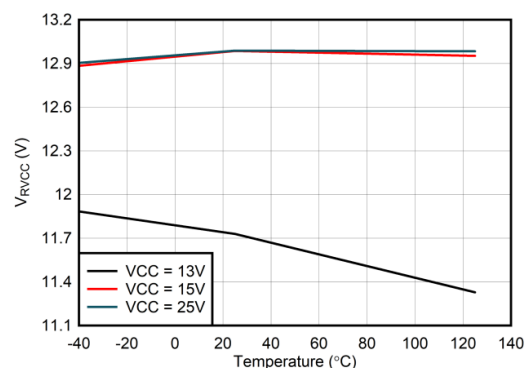
图 6-10. V_{\text{RVCC}} (100mA load) vs Temperature
