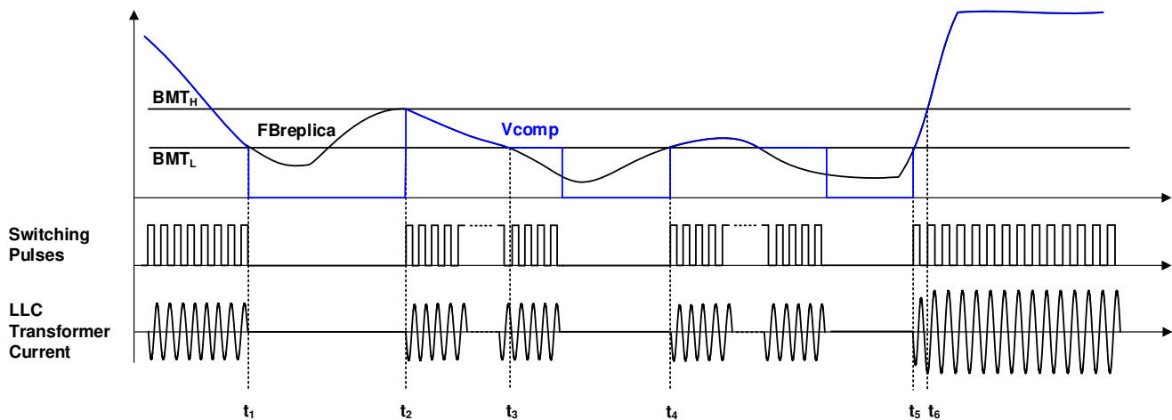
图 7-18. Burst Mode Switching Pattern when Soft On and Soft Off is Disabled
