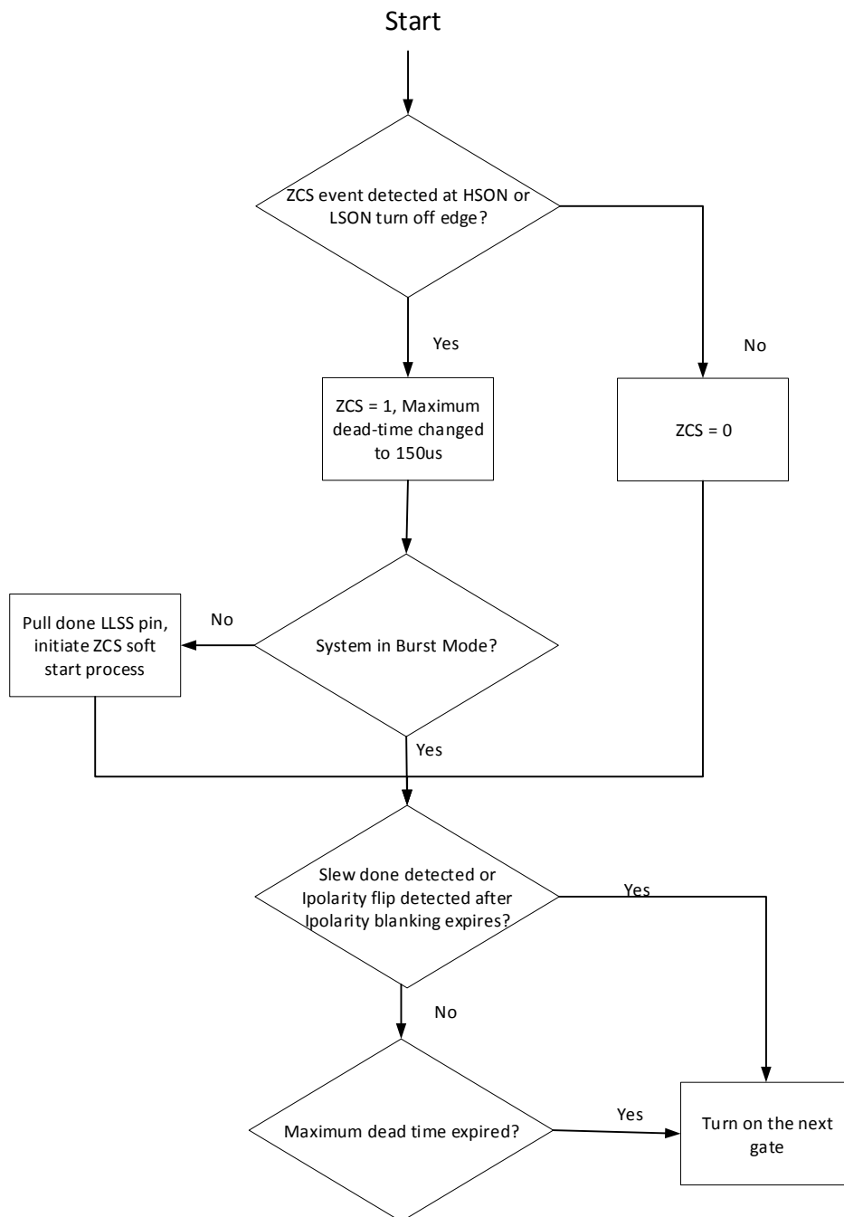
图 7-11. ZCS Prevention Algorithm Flow Chart
