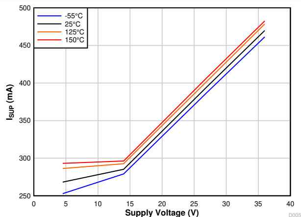
图 7-4. I_{SUP} Recessive vs V_{SUP} and Temperature
