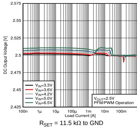
图 28. Output Voltage versus Load Current V_{OUT} = 2.5\text{ V}
