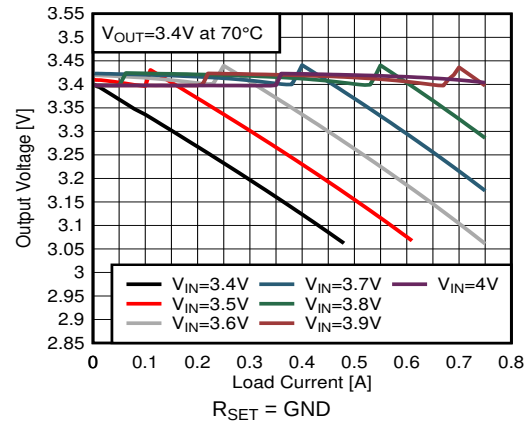
图 31. Output Voltage versus Load Current V_{OUT} = 3.4\text{ V}
