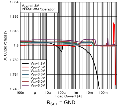
图 27. Output Voltage versus Load Current V_{OUT} = 1.8\text{ V}
