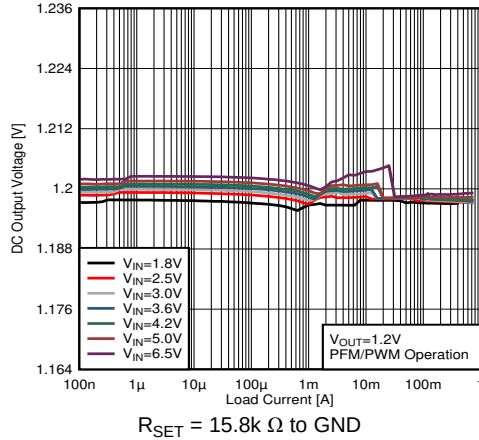
图 26. Output Voltage versus Load Current V_{OUT} = 1.2\text{ V}
