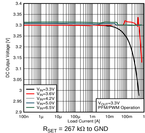
图 29. Output Voltage versus Load Current V_{OUT} = 3.3\text{ V}
