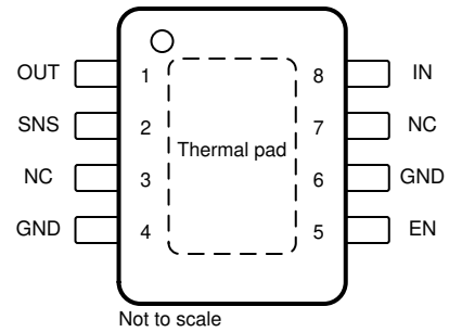
图 5-4. DGN Package (Fixed), 8-Pin HVSSOP, Top View
