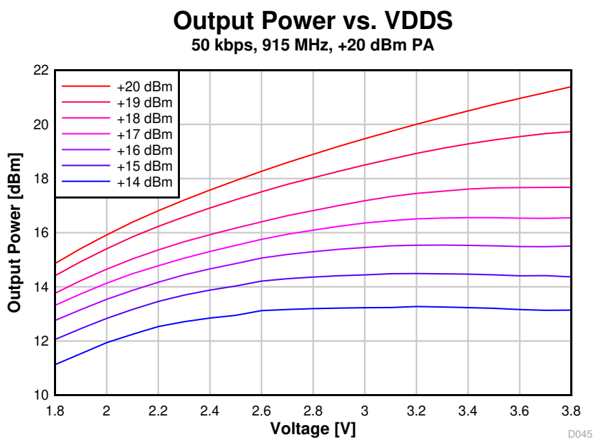
图 8-46. Output Power vs. Supply Voltage (VDDS) (50 kbps, 915 MHz)
