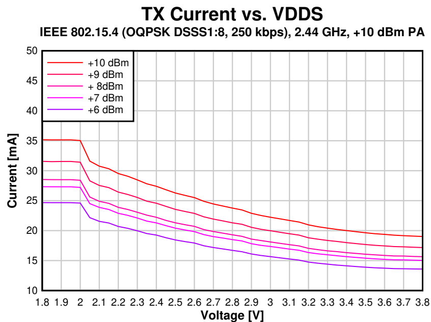
图 8-22. TX Current vs. Supply Voltage (VDD5) (250 kbps, 2.44 GHz, +10 dBm PA)
