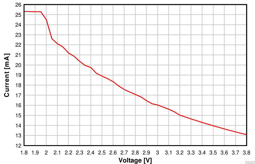
图 8-18. TX Current vs. Supply Voltage (VDD5) (50 kbps, 868.3 MHz)
