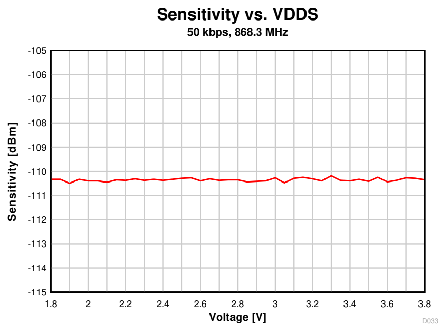
图 8-30. Sensitivity vs. Supply Voltage (VDD5) (50 kbps, 868.3 MHz)
