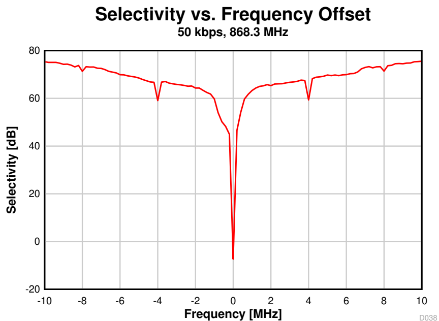
图 8-34. Selectivity vs. Frequency Offset (50 kbps, 868.3 MHz)
