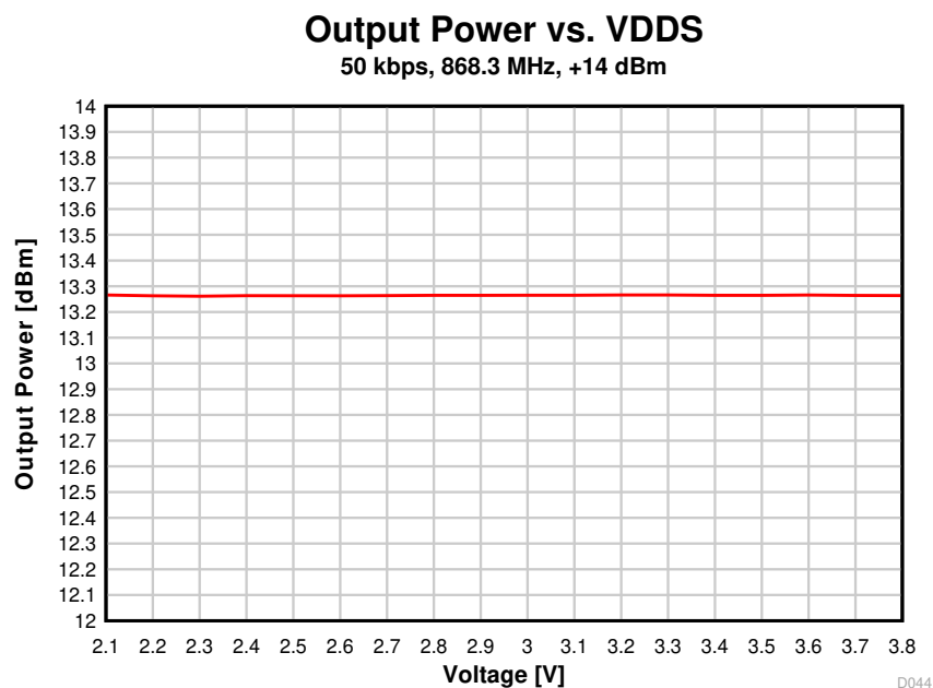
图 8-45. Output Power vs. Supply Voltage (VDDS) (50 kbps, 868.3 MHz)
