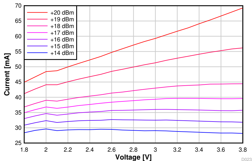
图 8-19. TX Current vs. Supply Voltage (VDD5) (50 kbps, 915 MHz)
