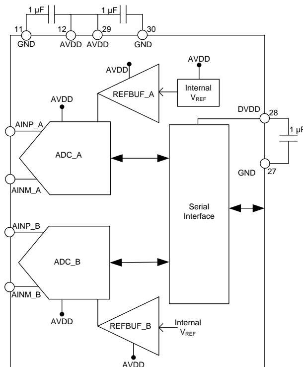
图 83. Power-Supply Decoupling
