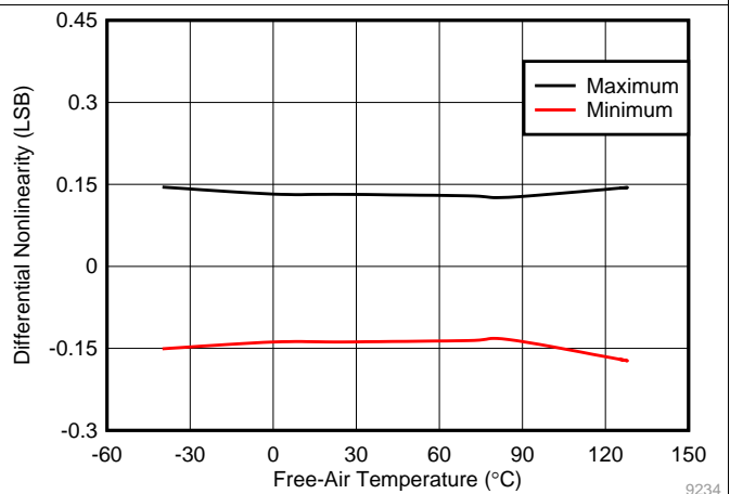
图 32. Typical DNL
