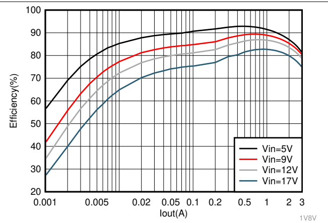
图 8. TPS563231 V_{OUT} = 1.8\text{ V} Efficiency
