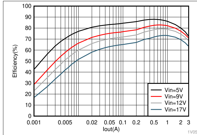
图 7. TPS563231 V_{OUT} = 1.05\text{ V} Efficiency
