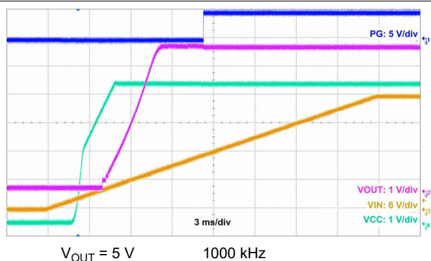
图 10-33. Start-Up Waveform
