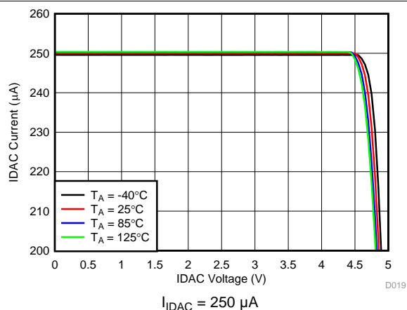
图 43. IDAC Current vs IDAC Voltage
