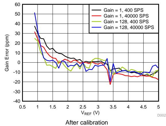
图 17. Gain Error vs Reference Voltage
