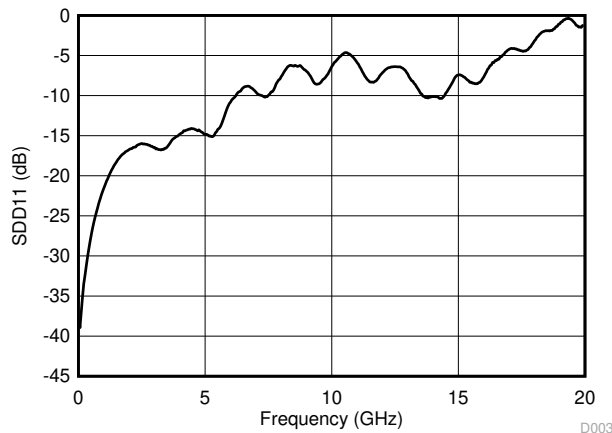
图 5-11. Input Return Loss Performance of the Upstream Ports
