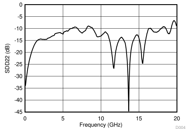
图 5-12. Output Return Loss Performance of the Upstream Ports
