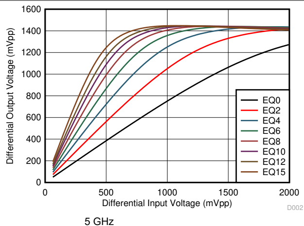
图 5-16. Upstream-to-Downstream Linearity Performance at 5 GHz
