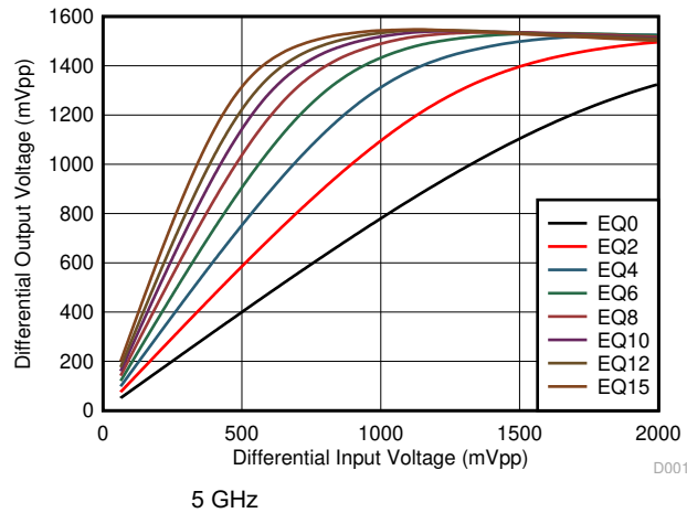
图 5-13. Downstream-to-Upstream Linearity Performance at 5 GHz
