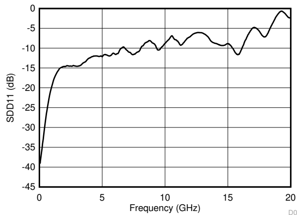
图 5-9. Input Return Loss Performance of the Downstream Ports
