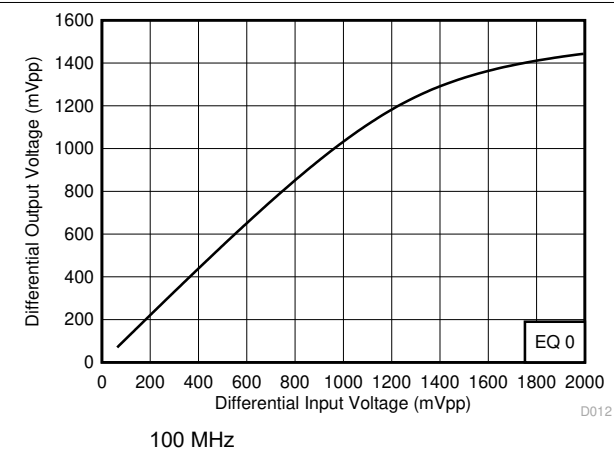
图 5-18. Upstream-to-Downstream Linearity Performance at 100 MHz
