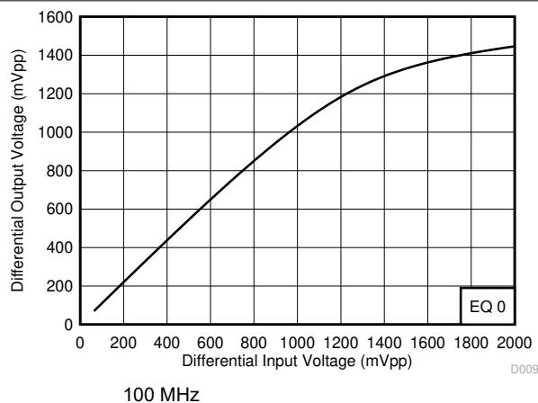
图 5-15. Downstream-to-Upstream Linearity Performance at 100 MHz
