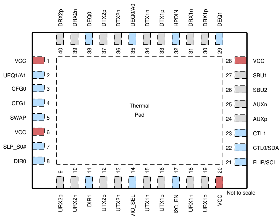
图 4-1. RNQ Package 40-Pin (WQFN) Top View
