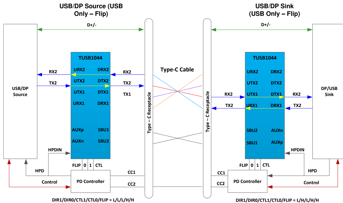
图 7-5. USB3.1 Only - With Flip
