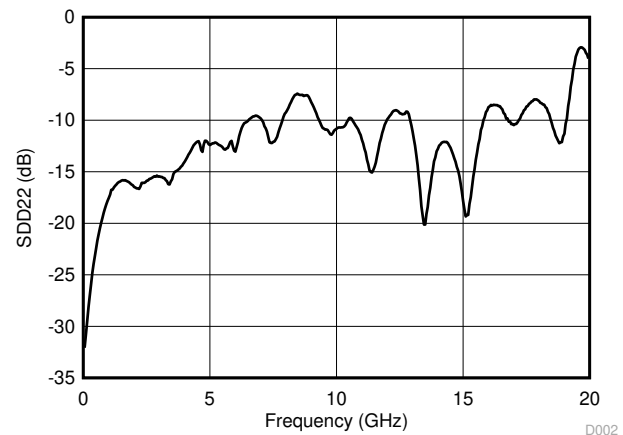
图 5-10. Output Return Loss Performance of the Downstream Ports
