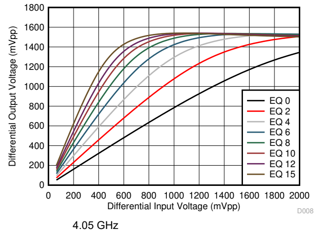
图 5-14. Downstream-to-Upstream Linearity Performance at 4.05 GHz
