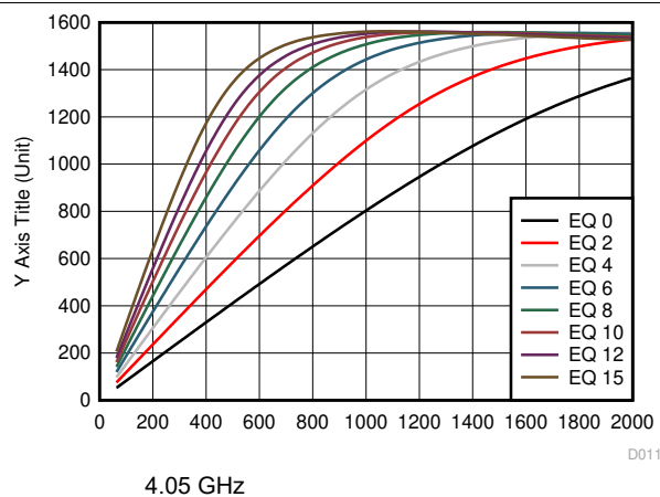
图 5-17. Upstream-to-Downstream Linearity Performance at 4.05 GHz
