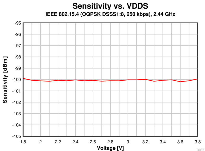
图 8-27. Sensitivity vs. Supply Voltage (VDDS) (250 kbps, 2.44 GHz)
