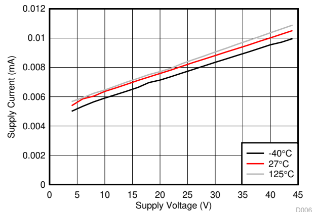
图 7-6. Standby Recessive I_{SUP} vs V_{SUP} and Temperature
