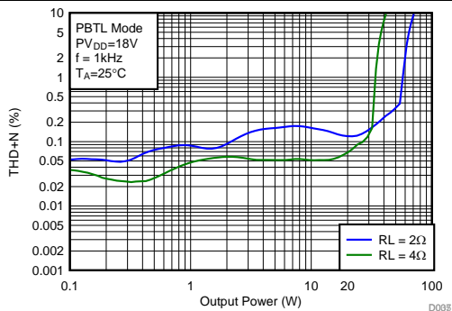
图 34. Total Harmonic Distortion + Noise vs Output Power (PBTL Mode)
