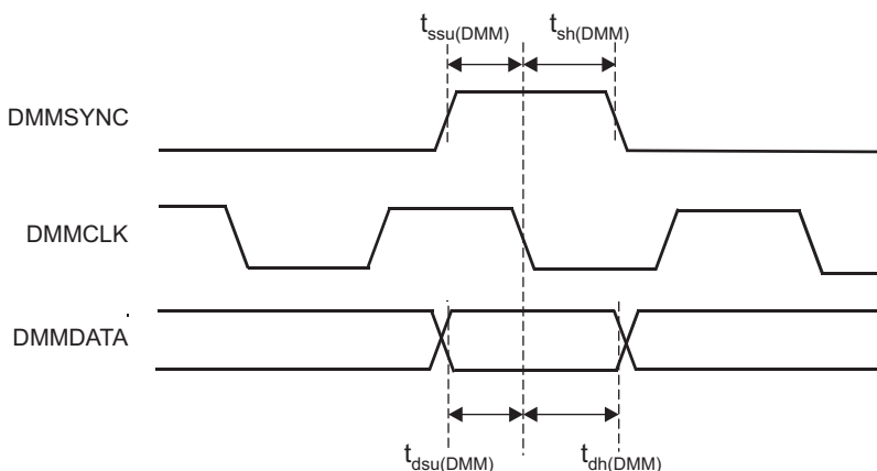
Figure 5-19. DMMDATA Timing
