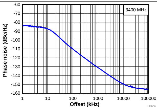
图 10. Narrow Band Phase Noise at 3.4 GHz
