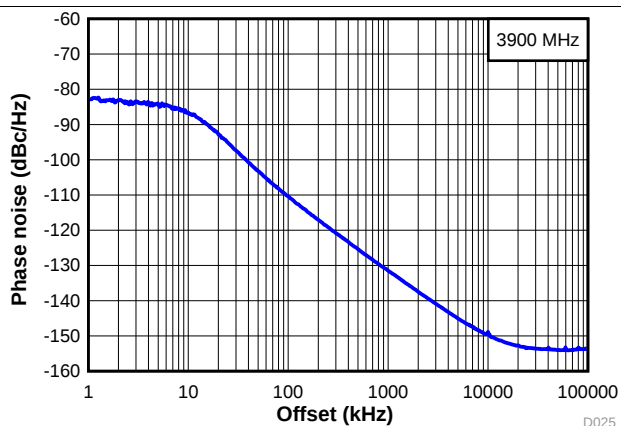
图 12. Narrow Band Phase Noise at 3.9 GHz
