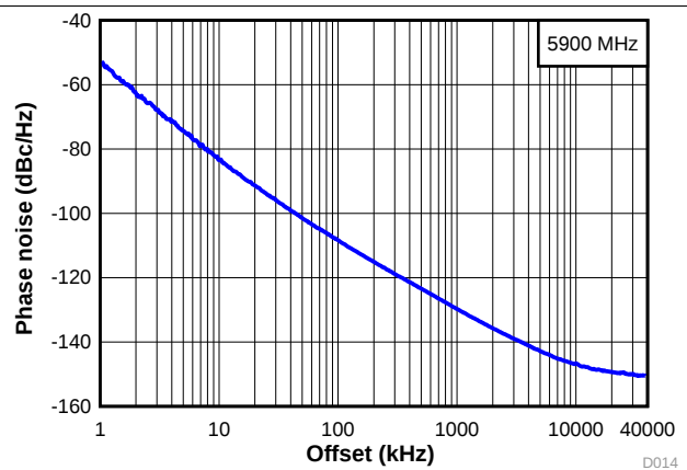
图 8. Open-Loop VCO Phase Noise at 5.9 GHz
