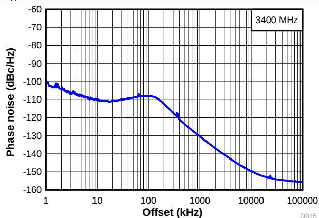
图 9. Wide Band Phase Noise at 3.4 GHz
