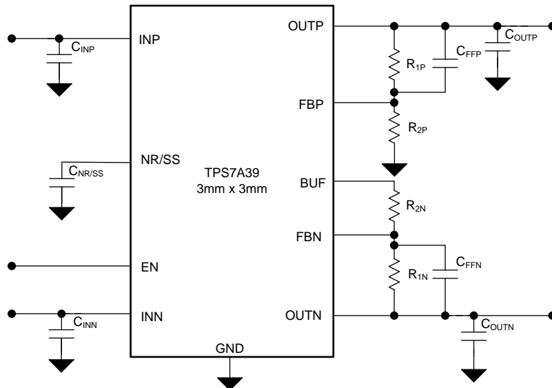
图 65. Adjustable Operation
