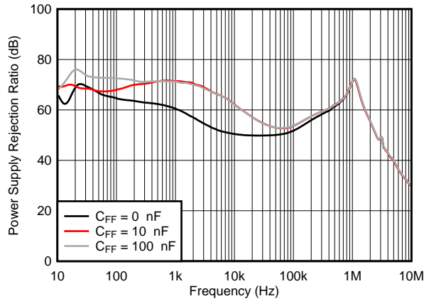
图 8. Positive PSRR vs Frequency and C_{FFP}
