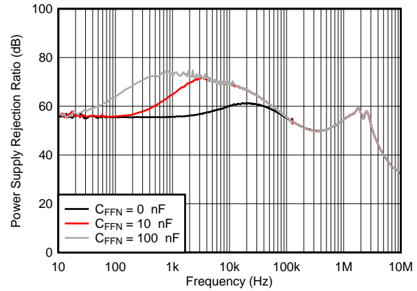
图 9. Negative PSRR vs Frequency and C_{FFN}
