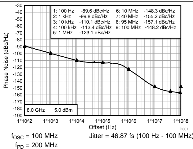
Figure 7. Closed-Loop Phase Noise at 8 GHz
