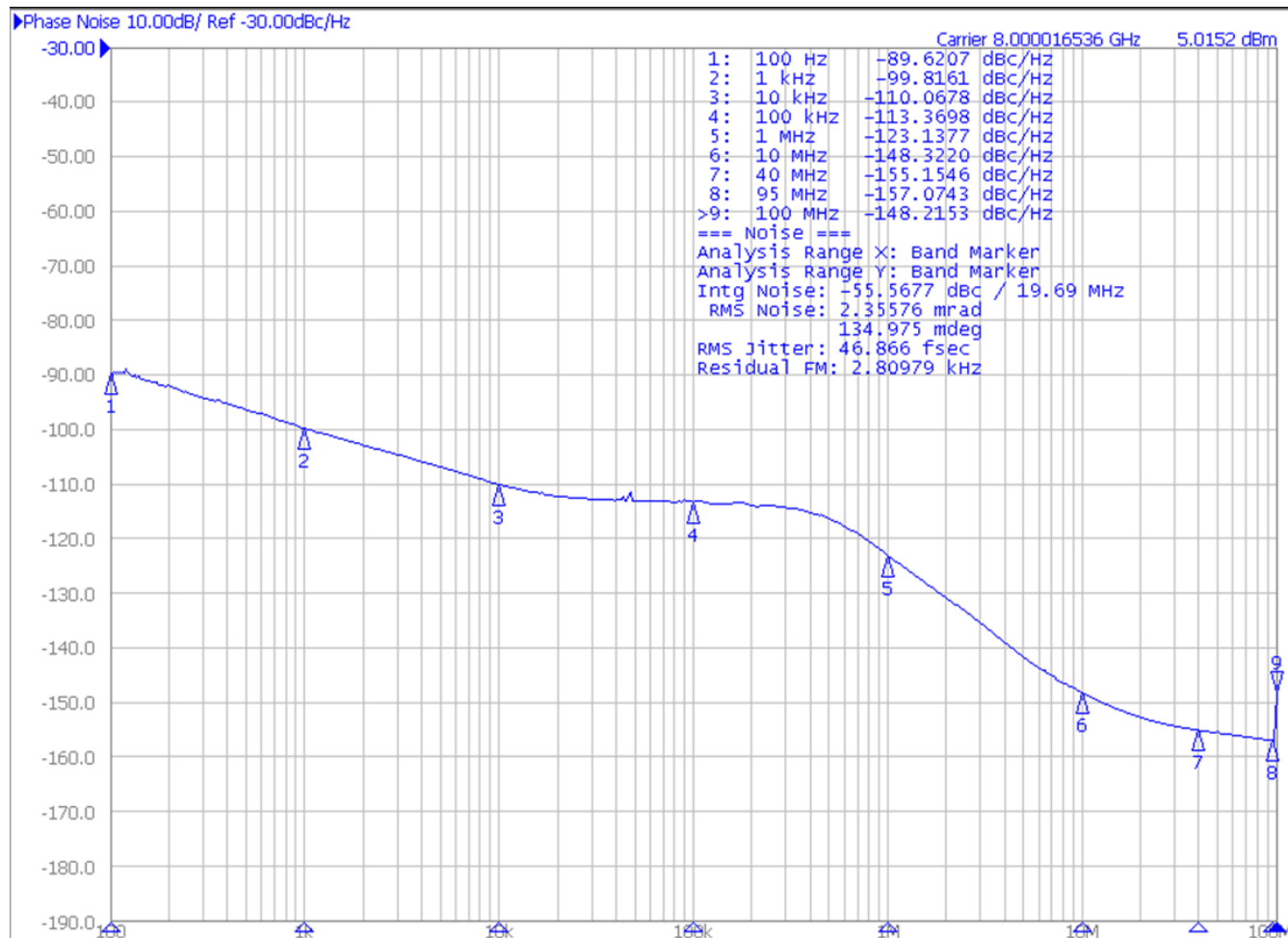
Figure 53. Typical Jitter
