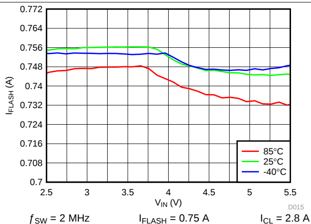
图 16. LED Flash Current vs Input Voltage
