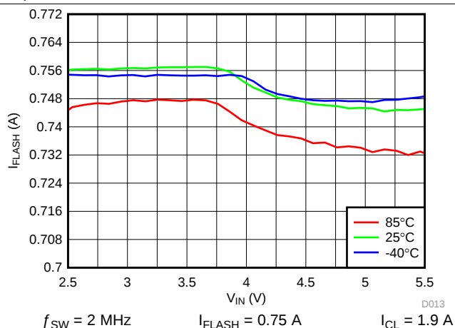
图 14. LED Flash Current vs Input Voltage
