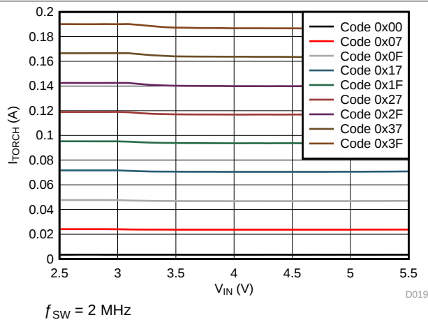
图 20. LED Torch Current vs Input Voltage
