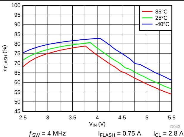
图 53. LED Flash Efficiency vs Input Voltage
