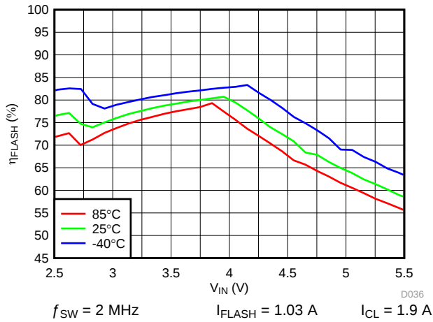
图 46. LED Flash Efficiency vs Input Voltage
