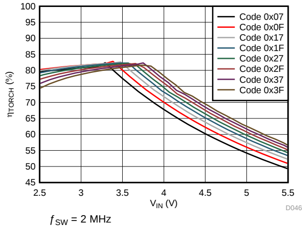
图 56. LED Torch Efficiency vs Input Voltage
