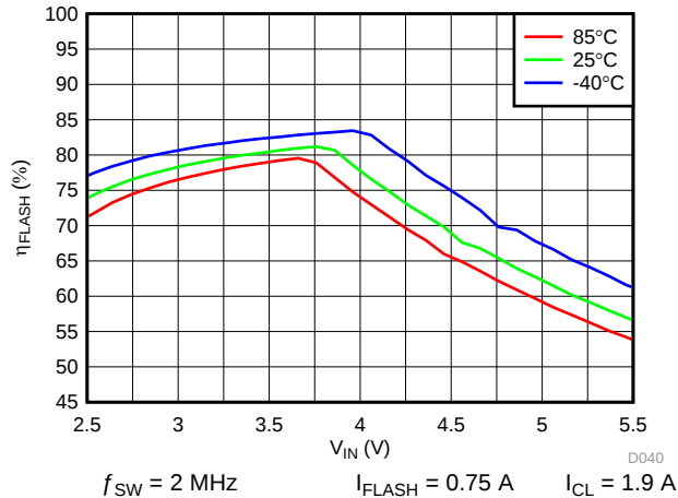
图 50. LED Flash Efficiency vs Input Voltage
