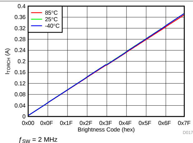
图 18. LED Torch Current vs Brightness Code
