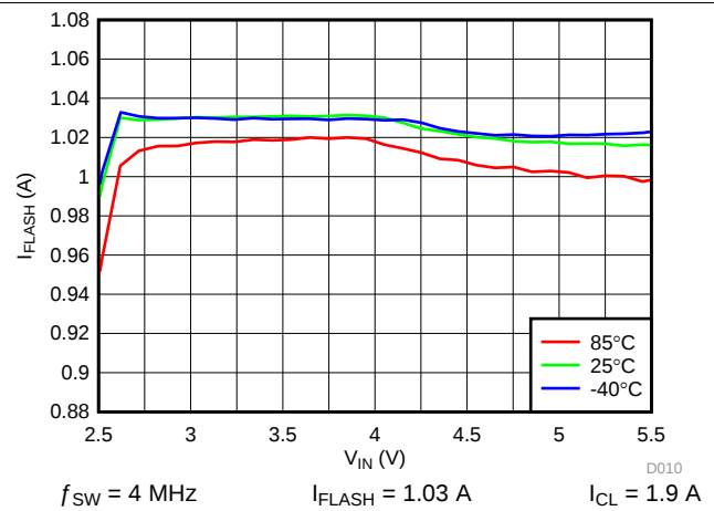
图 11. LED Flash Current vs Input Voltage
