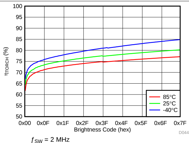
图 54. LED Torch Efficiency vs Brightness Code
