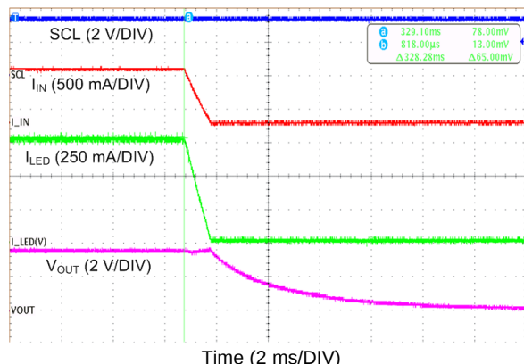
Time (2 ms/DIV)
