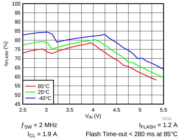
图 44. LED Flash Efficiency vs Input Voltage
