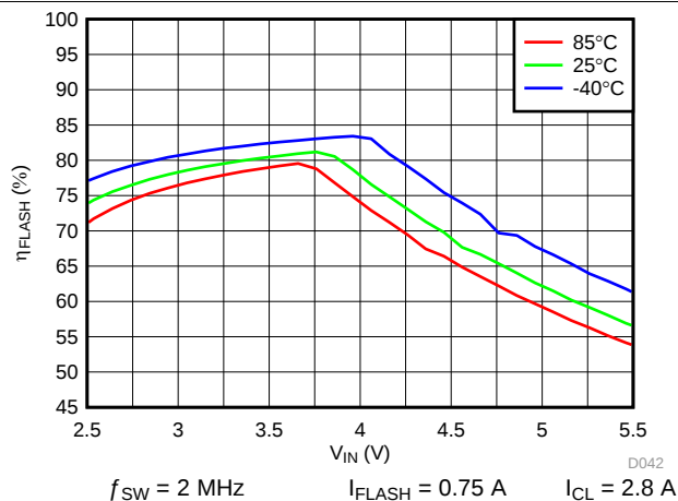
图 52. LED Flash Efficiency vs Input Voltage
