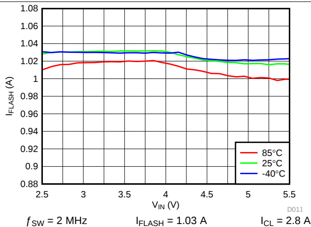
图 12. LED Flash Current vs Input Voltage
