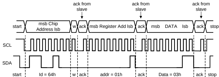
图 35. Write Cycle W = Write (SDA = 0) R = Read (SDA = 1) Ack = Acknowledge (SDA Pulled Down by Either Master or Slave) ID = Chip Address, 64h for LM36010
