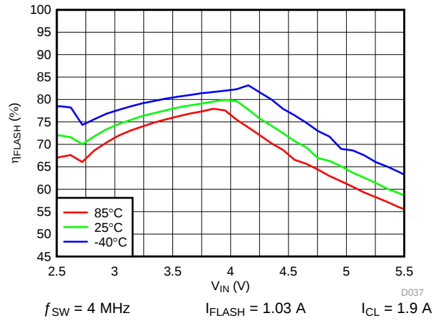
图 47. LED Flash Efficiency vs Input Voltage
