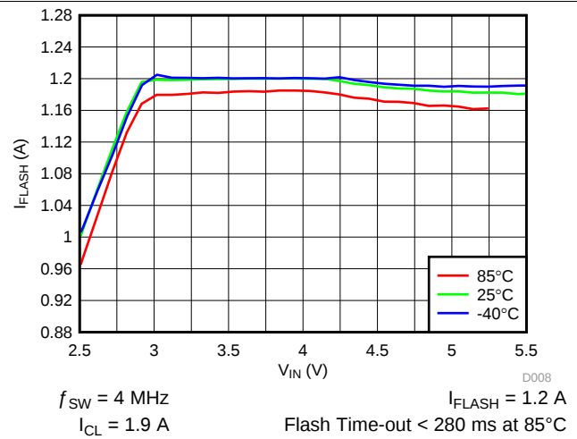
图 9. LED Flash Current vs Input Voltage
