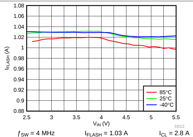
图 13. LED Flash Current vs Input Voltage
