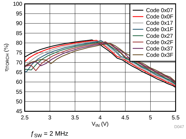
图 57. LED Torch Efficiency vs Input Voltage
