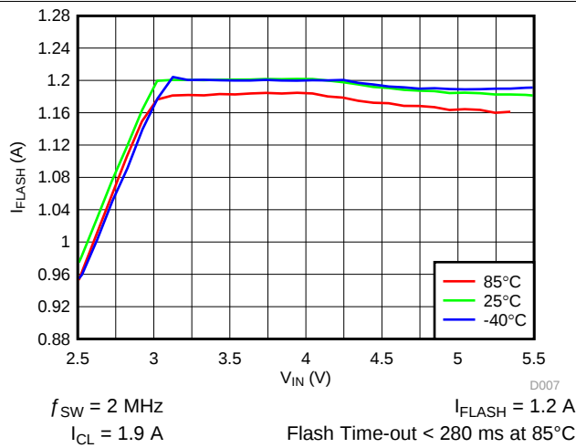
图 8. LED Flash Current vs Input Voltage
