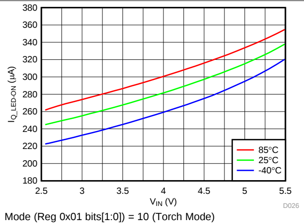
图 27. LED On Current vs Input Voltage
