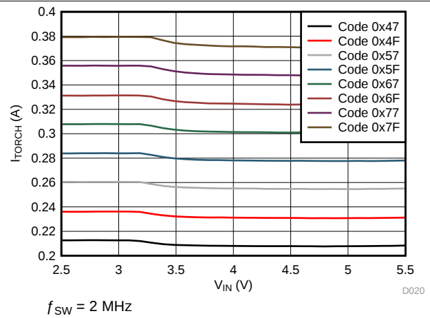
图 21. LED Torch Current vs Input Voltage
