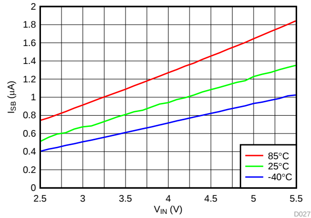
图 26. LED Off Current vs Input Voltage
