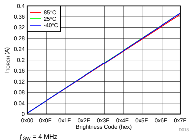
图 19. LED Torch Current vs Brightness Code
