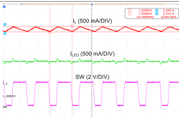
图 77. Pass mode Level Triggered Flash
