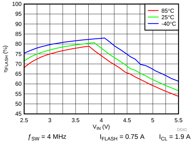
图 51. LED Flash Efficiency vs Input Voltage
