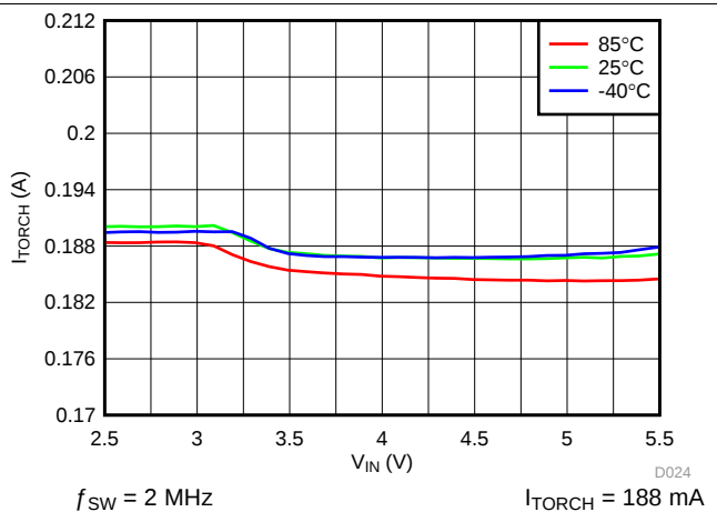
图 25. LED Torch Current vs Input Voltage
