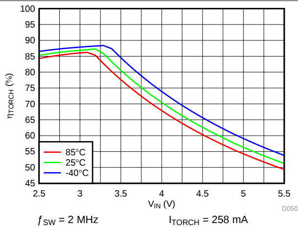
图 60. LED Torch Efficiency vs Input Voltage
