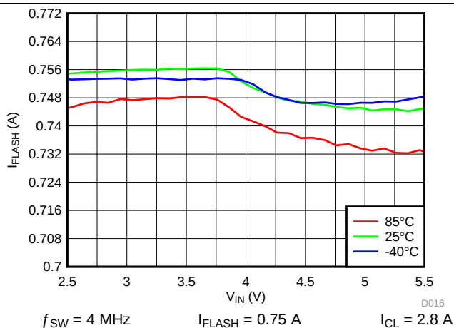
图 17. LED Flash Current vs Input Voltage
