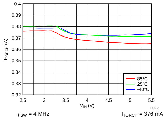
图 23. LED Torch Current vs Input Voltage
