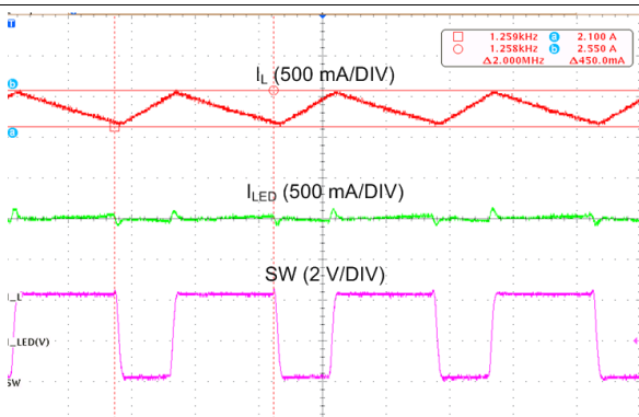
图 76. Pass mode Edge Triggered Flash
