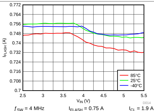
图 15. LED Flash Current vs Input Voltage
