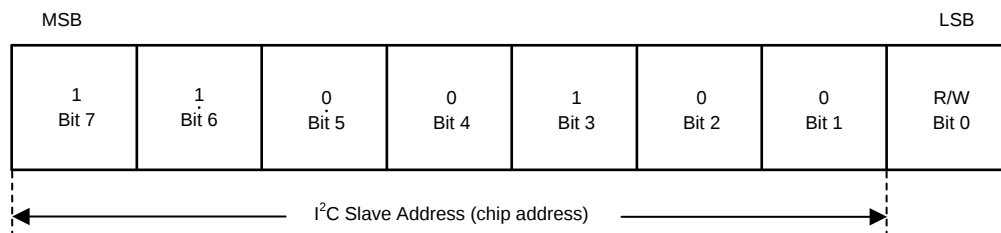
图 36. I 2 C-Compatible Chip Address
