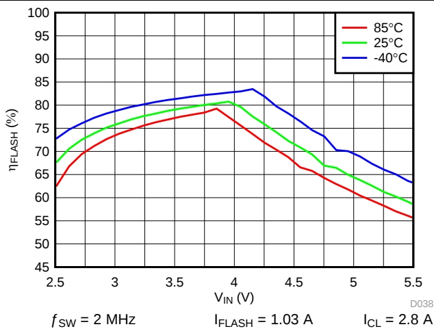
图 48. LED Flash Efficiency vs Input Voltage
