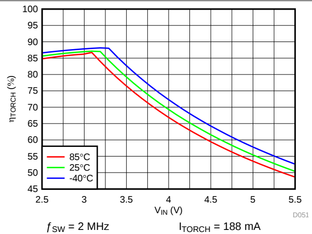
图 61. LED Torch Efficiency vs Input Voltage
