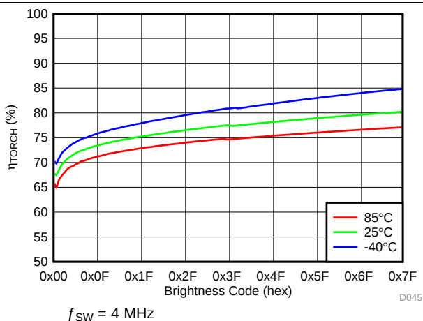
图 55. LED Torch Efficiency vs Brightness Code
