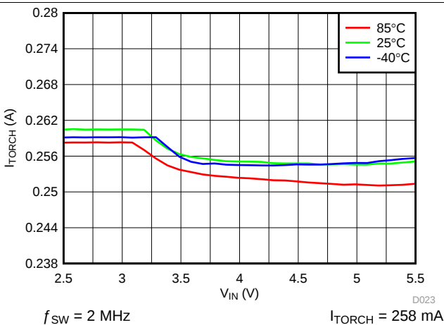
图 24. LED Torch Current vs Input Voltage
