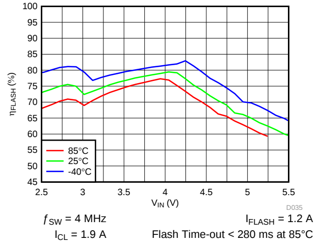
图 45. LED Flash Efficiency vs Input Voltage
