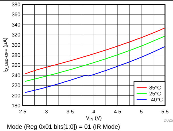
图 26. LED Off Current vs Input Voltage
