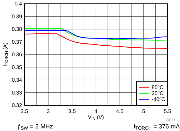
图 22. LED Torch Current vs Input Voltage
