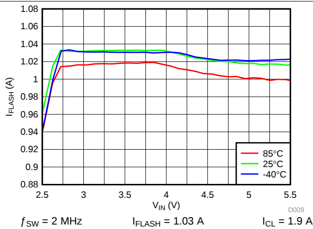
图 10. LED Flash Current vs Input Voltage
