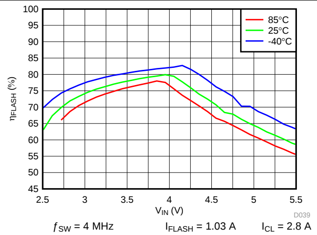
图 49. LED Flash Efficiency vs Input Voltage
