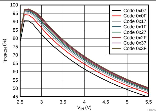
图 33. LED Torch Efficiency vs Input Voltage
