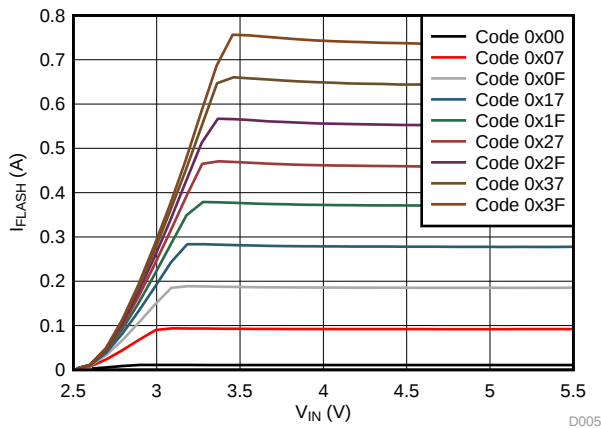
图 4. LED Flash Current vs Input Voltage
