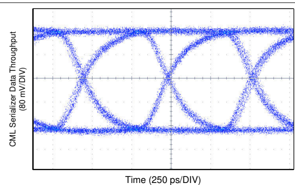
图 8-7. Coax Eye Diagram at 1.87-Gbps Line Rate (100-MHz Pixel Clock, 12-bit Mode) from Serializer Output (DOUT+)
