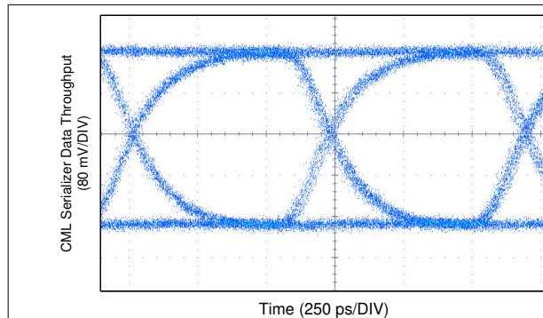
图 8-6. Coax Eye Diagram at 1.4-Gbps Line Rate (100-MHz Pixel Clock, 10-bit Mode) from Serializer Output (DOUT+)
