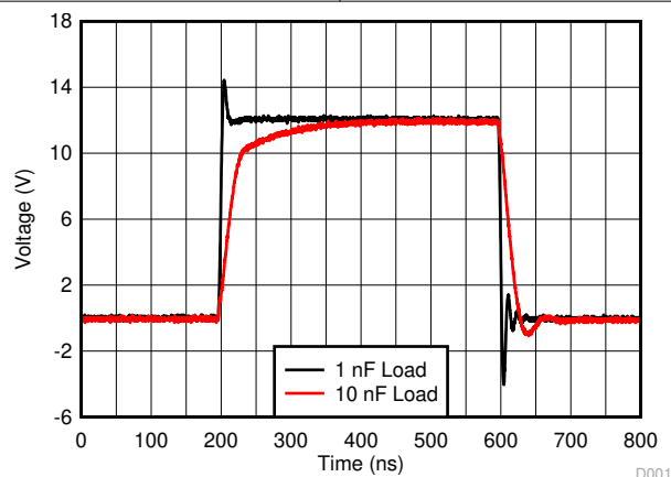
图 6-24. Typical Output Voltage
