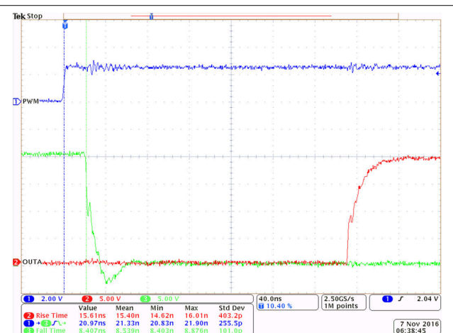
图 9-6. Zoomed-In bench-test waveform
