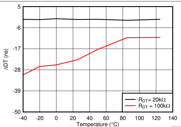
图 6-23. Dead Time Matching vs. Temperature
