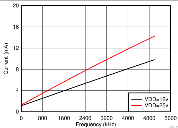
图 6-4. Per Channel Current Consumption vs. Frequency
