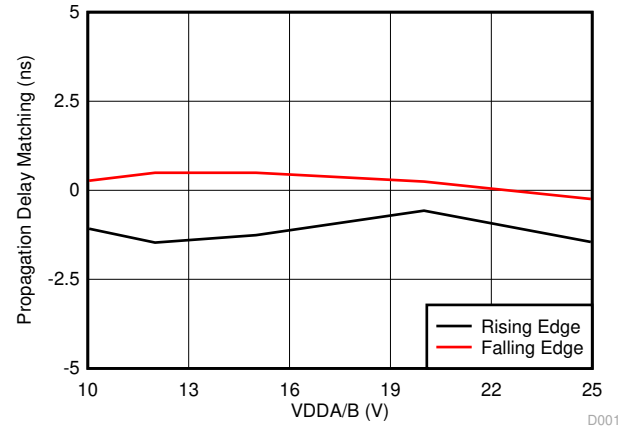
图 6-15. Propagation Delay Matching ( t_{DM} ) vs. VDD
