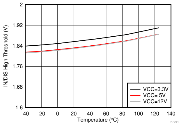
图 6-21. PWM/DIS High Threshold
