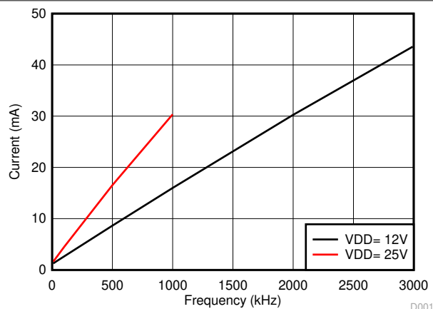
图 6-5. Per Channel Current Consumption (I VDDA/B ) vs. Frequency
