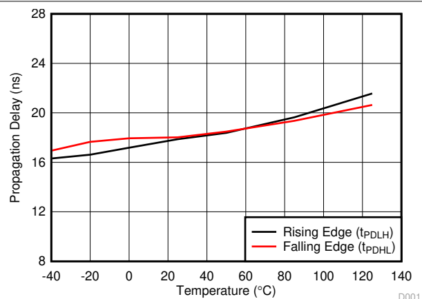
图 6-12. Propagation Delay vs. Temperature
