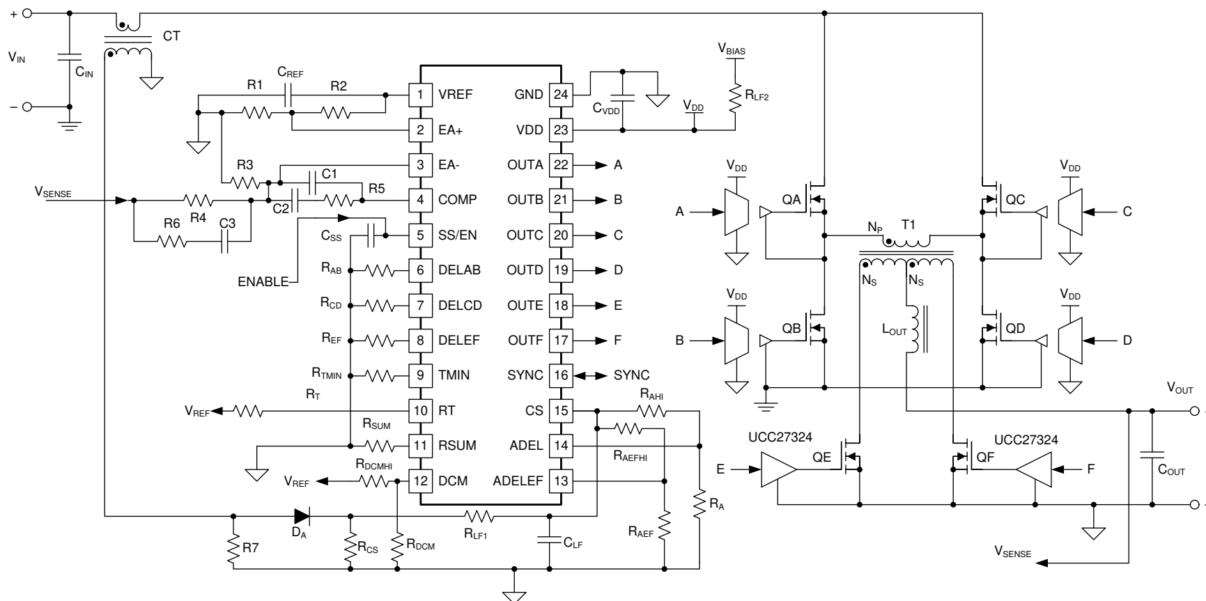
图 7-3. Typical Application
