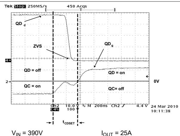
图 7-16. Full-Bridge Gate Drives and Switch Nodes (QD g QD d )
