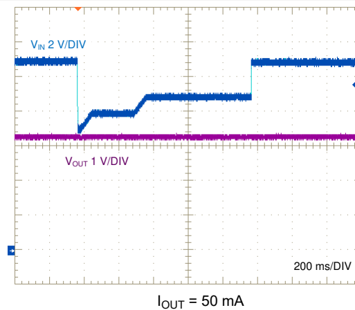
图 8-20. Input Voltage Transient (Automotive Cold Crank Profile)
