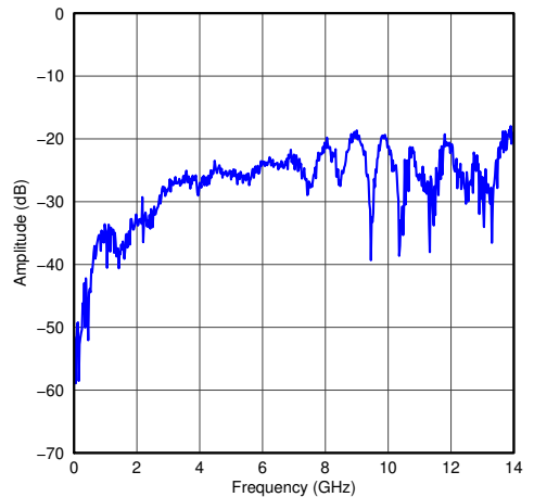
图 6-2. Differential to Common Mode Conversion
