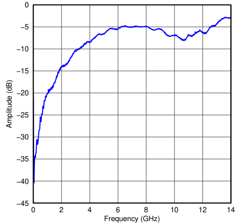
图 6-4. Common Mode Output Return Loss
