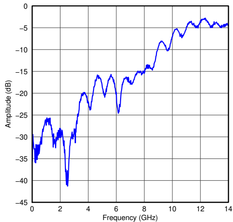
图 6-1. Differential Input Return Loss
