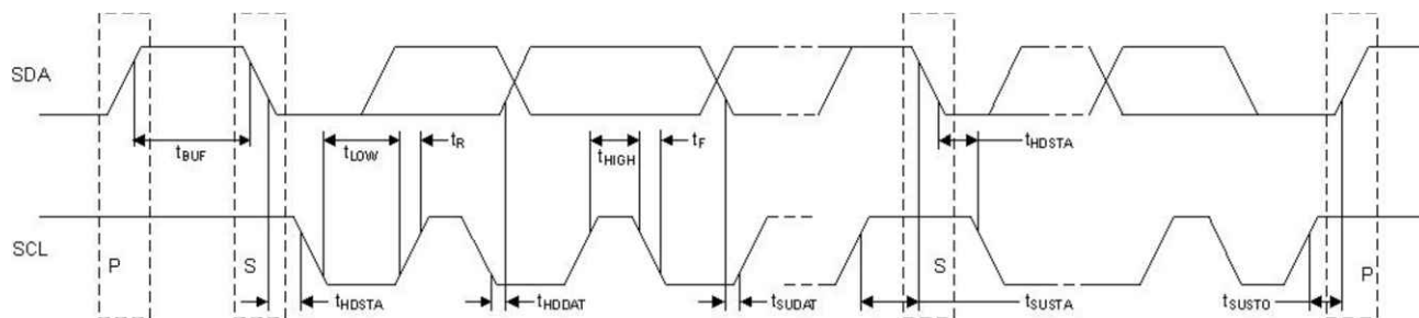
图 7-11. Two - Wire Serial Interface Timing Diagram
