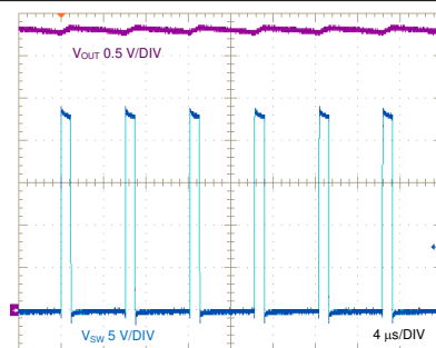
图 8-28. SW Node and Output Ripple Voltages, Full Load
