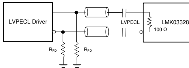
图 8-12. AC-Coupling LMK03328 Inputs With LVPECL Signal
