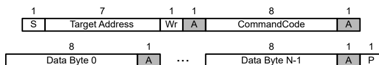
图 8-34. Block Register Write Programming Sequence
