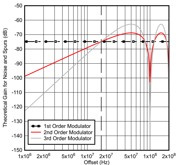
图 8-19. Theoretical Delta Sigma Noise Shaping for a 100-MHz Phase Detector Frequency
