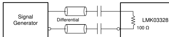
图 7-12. Differential Input AC Configuration During Device Test
