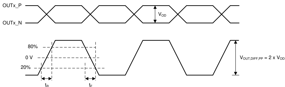
图 7-15. Differential Output Voltage and Rise/Fall Time
