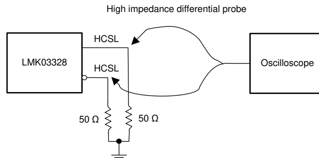
图 7-4. HCSL Output DC Configuration During Device Test
