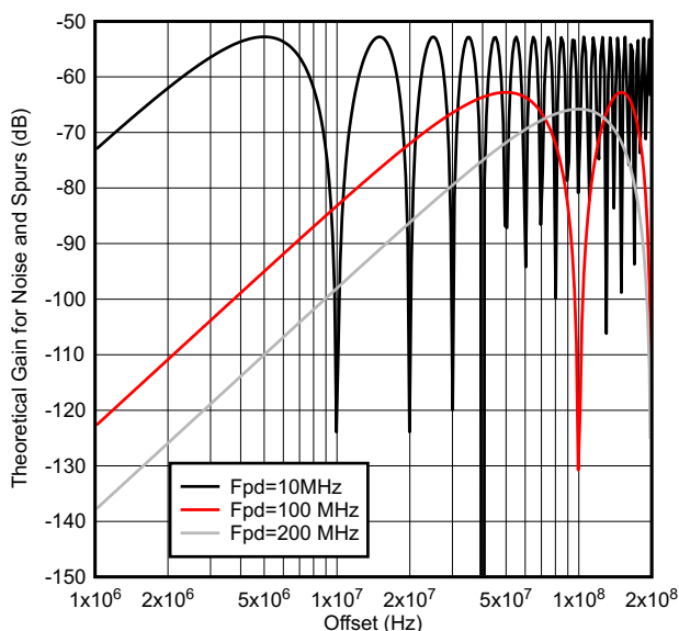
图 8-20. Theoretical Delta Sigma Noise Shaping for 3rd Order Modulator
