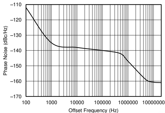
图 6-9. Closed-Loop Phase Noise of HCSL Outputs at 161.1328125 MHz With PLL Bandwidth at 400 kHz, Fractional N PLL, 50-MHz Crystal Input, 5-GHz VCO Frequency, Post Divider = 8, Output Divider = 4
