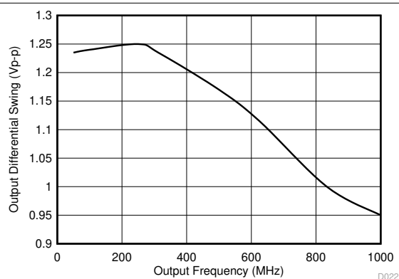
图 6-20. AC-CML Differential Output Swing vs. Frequency
